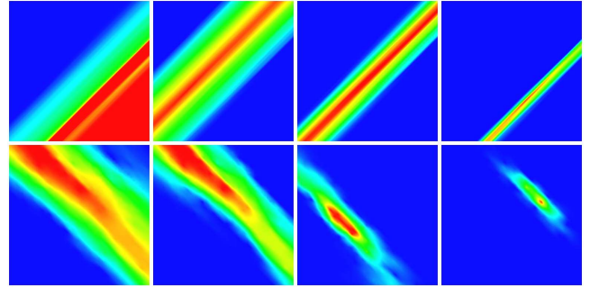
Figure 17: For the two vector fields v_1 = (-1, 1) (bottom row) and v_2 = (1, 1) (top row) basis functions on the four coarsest levels are shown. Obviously the basis functions are clearly aligned to the flow field (cf. Fig. 16).
