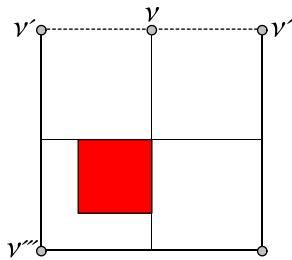
Figure 7.4 Node v is L -useful for L < 3 because L * (1 + 1) < 6 and edge \epsilon(v, v'''' ) \in C_{\text{forb}} . If the value for L is less than three, then node v and edges \epsilon(v, v') and \epsilon(v, v'' ) are added to the graph, introducing a useful cycle.
