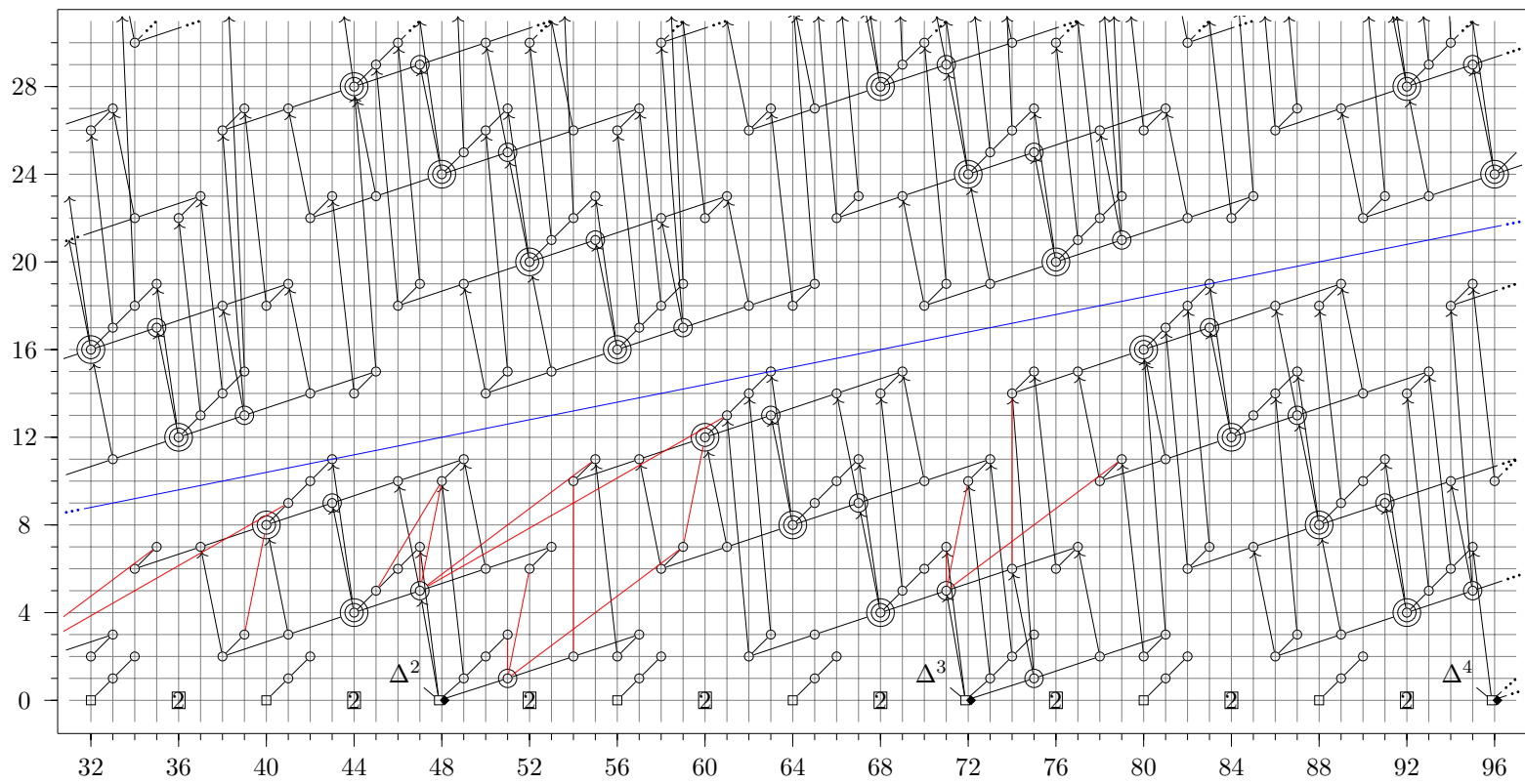
Figure A.4: The DSS for Tmf_{(2)} from the E_5 -page in the range 32 \leq n \leq 96 .
