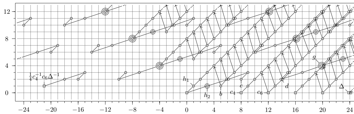
Figure A.2: E_3 -page of the DSS for \mathrm{Tmf}_{(2)} .
