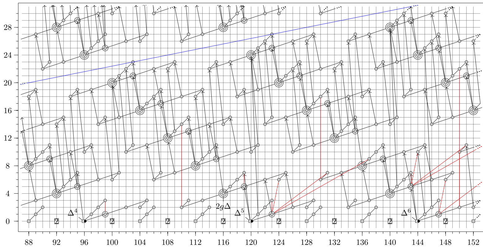
Figure A.5: The DSS for Tmf_{(2)} from the E_5 -page in the range 88 \leq n \leq 152 .
