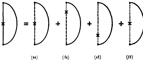
Fig. 7. Decomposition of the operator B_{(A)}^s(t) occurring in diagrams of subclass IV A.
