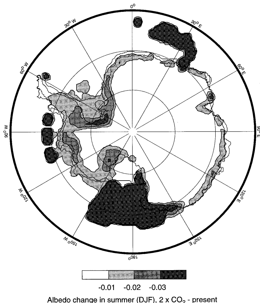
FIG. 13. Modeled change of surface albedo for the summer (DJF), 2 \times \text{CO}_2 -present. The pattern of summer albedo change shows essentially two effects in the 2 \times \text{CO}_2 climate run. The first is the removal of sea ice at some places, leading to a dramatic drop in albedo from the sea-ice value (0.5–0.75) to that of sea water (0.065). These changes are visible as dark blobs. The second effect, which is of most interest here, are the more subtle changes that result from the temperature increase above the threshold for albedo changes (i.e., -10^\circ\text{C} ) over the coastal zone of the ice sheet.
