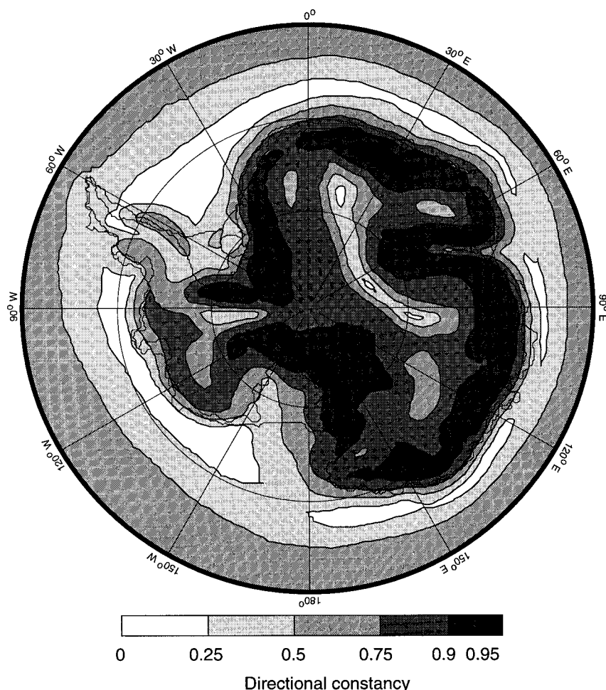
FIG. 11. Modeled distribution of annual mean directional constancy dc .
