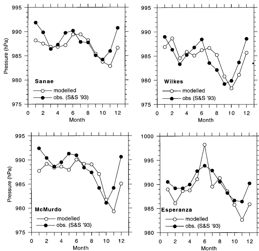
FIG. 6. Observed (black dots) and modeled (white dots) annual cycle of sea level pressure at four Antarctic stations. Abbreviated data source: S&S '93, Smith and Stearns (1993).
