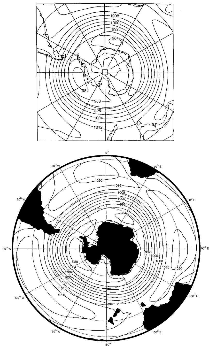
FIG. 3. Observed (a) and modeled (b) average summer (DJF) sea level pressure distribution; observed (c) and modeled (d) average winter (JJA) sea level pressure distribution. The observations are 10-yr mean distributions of UKMO data assimilation, taken from Connolley and Cattle (1994).
