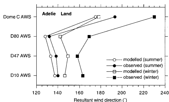
FIG. 10. Observed (black symbols) and modeled (white symbols) resultant wind direction at four AWS in Adélie Land. Squares denote winter (JJA) and circles summer (DJF) wind directions. Observations from Kodama and Wendler (1986).
