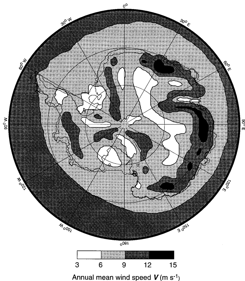
FIG. 8. Modeled distribution of annual mean 10-m wind speed.
