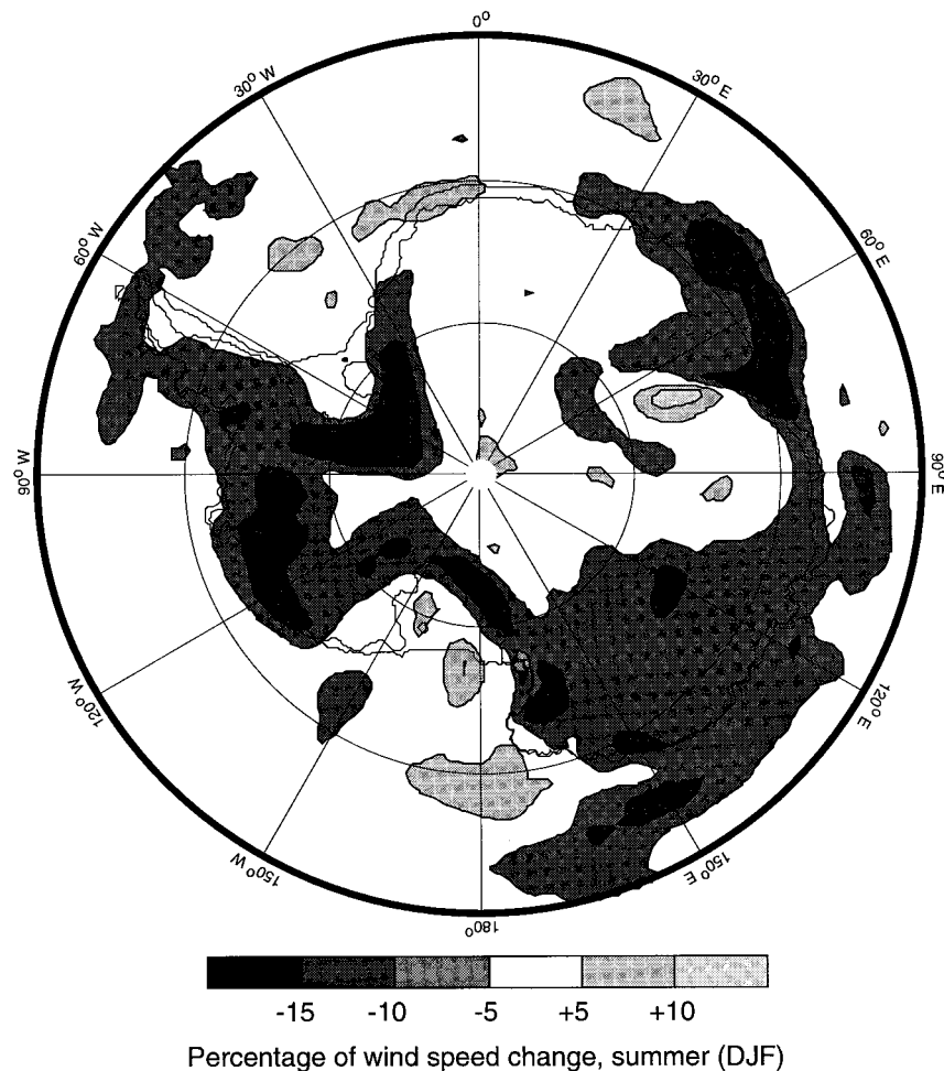
FIG. 12. Modeled relative change ( 2 \times \text{CO}_2 -present) of 10-m wind speed for (a) summer months (DJF) and (b) winter months (JJA).
