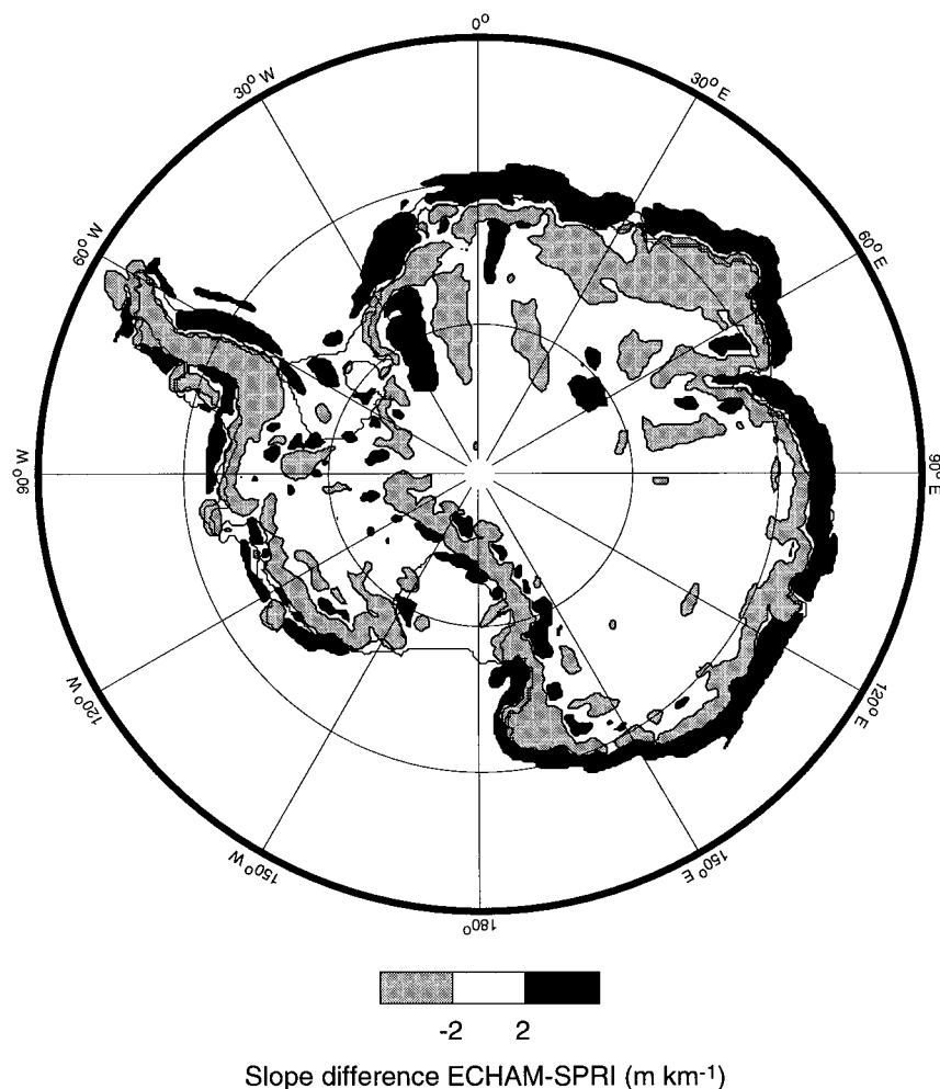
FIG. 2. Difference in surface slope between ECHAM and SPRI data. Areas where ECHAM - SPRI < -2 \text{ m km}^{-1} are light shaded, ECHAM - SPRI > 2 \text{ m km}^{-1} dark shaded.
