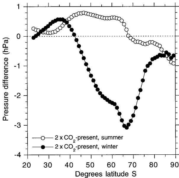
FIG. 14. Modeled change of zonally averaged sea level pressure, 2 \times \text{CO}_2 -present, for summer months (white dots) and winter months (black dots).
