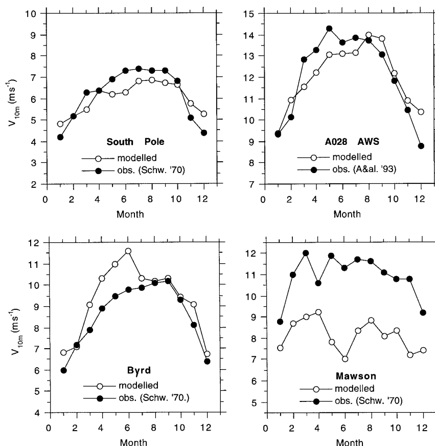
FIG. 9. Observed (black dots) and modeled (white dots) annual cycle of 10-m wind speed at four Antarctic stations. Abbreviated data sources: Schw. '70, Schwerdtfeger (1970); A&al. '93, Allison et al. (1993).
