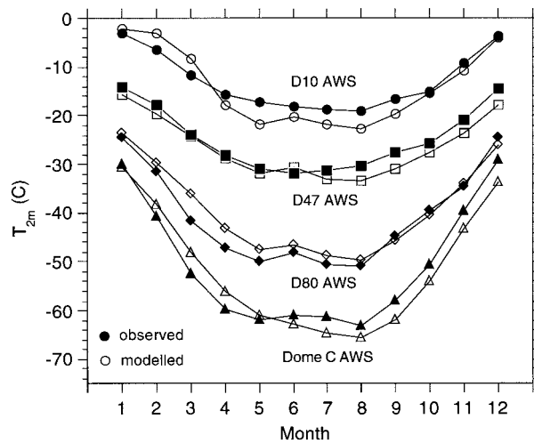
FIG. 7. Observed (black symbols) and modeled (white symbols) annual cycle of near-surface temperature at four Antarctic AWSs in Adélie Land. Observations from Allison et al. (1993).
