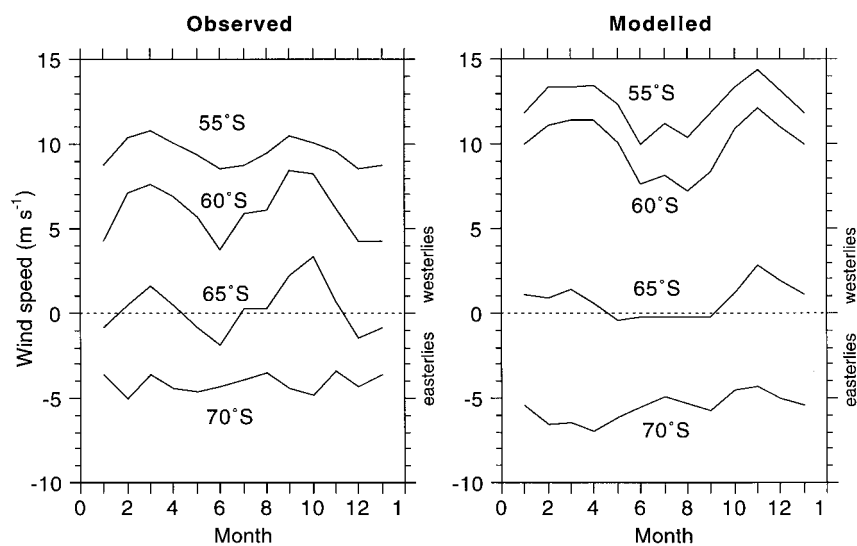
FIG. 5. Observed (van Loon et al. 1971) (left) and modeled (right) annual cycle of the zonal geostrophic wind speed, zonally averaged. Positive values indicate westerlies; negative values easterlies.
