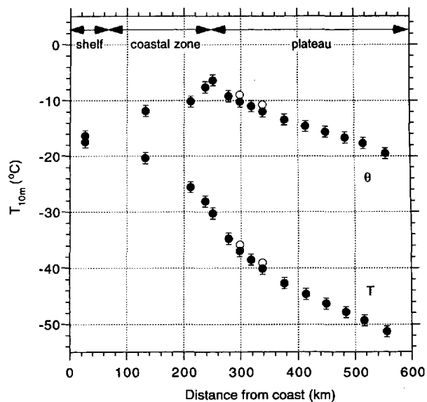
Fig. 3. Absolute and potential temperature at 10 m depth in the firn. White dots indicate uncorrected temperatures at sites E and G. Error bars indicate \pm 1 standard error.
