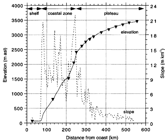
Fig. 2. Surface elevation (solid line) and terrain slope (dashed line). For the calculation of distance to the coast ( x axis), the coastline is assumed to be 70° S. Drilling locations are indicated by triangles.
