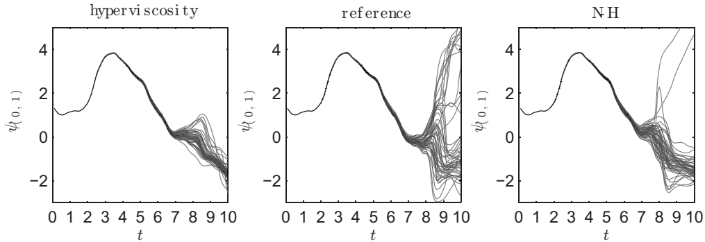
FIGURE 6. Ensemble dispersion in a classical double cascade. Plotted is the phase angle of the (0,1)-mode using (left) the model with Hyperviscosity, (centre) the Reference simulation, and (right) the Nosé-Hoover method as indicated with † in table 1.
