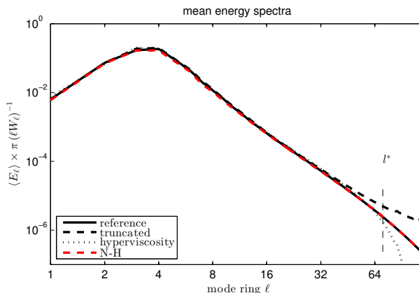
FIGURE 2. The kinetic energy spectrum, averaged over 100 time units, for the Reference (solid), a Truncated (dashed), Hyperviscosity (dotted) and Nosé-Hoover (dashed, red) configurations. Parameters are given in table 1, where the † indicates the parameters used here for the Nosé-Hoover control.
