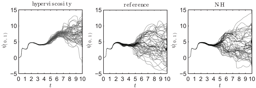
FIGURE 10. Ensemble dispersion in a simulation with small scale forcing. Plotted is the phase angle of the (0,1)-mode using (left) the model with Hyperviscosity, (centre) the Reference simulation, and (right) the Nosé-Hoover as indicated with † in table 1.
