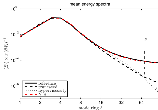
FIGURE 7. The kinetic energy spectrum after 100 time units for the Reference (solid), Truncated (dashed), Hyperviscosity (dotted) and Nosé-Hoover (dashed, red) configurations. Parameters are given in table 1, where the † indicates the parameters used here for the Nosé-Hoover control. An additional forcing is applied to the wavenumbers 203.5 < |\mathbf{k}| < 206.5 , with a power injection equal to that of the large scale forcing.
