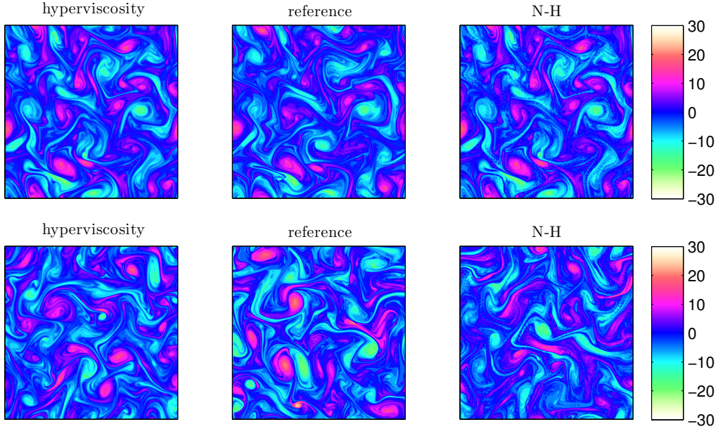
FIGURE 4. Vorticity fields in a classical double cascade, obtained at t = 1 (top) and t = 10 (bottom) using (left) the model with added Hyperviscosity, (centre) the Reference simulation, and (right) the Nosé-Hoover method as indicated with † in table 1.
