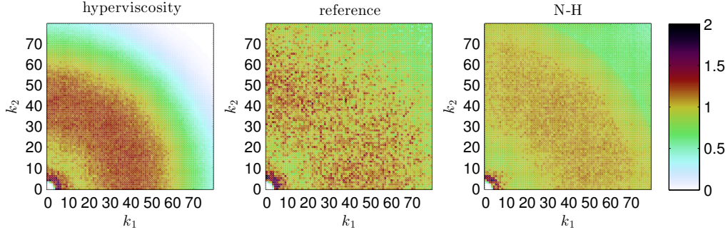
FIGURE 3. A representation of the time-averaged energy in each Fourier mode using (left) the Hyperviscosity model, (centre) the Reference simulation, and (right) the Nosé-Hoover control, see table 1 for details. The value plotted is given by \hat{C}_k = 2\pi\overline{\omega_k\omega_k^*}/(C'\eta^{2/3}k^{-3-d-1}) , where the parameters C' and d are fit to the reference solution (cf. 2.8). When this value is close to unity, it indicates close local (in Fourier space) agreement to the power-law spectrum.
