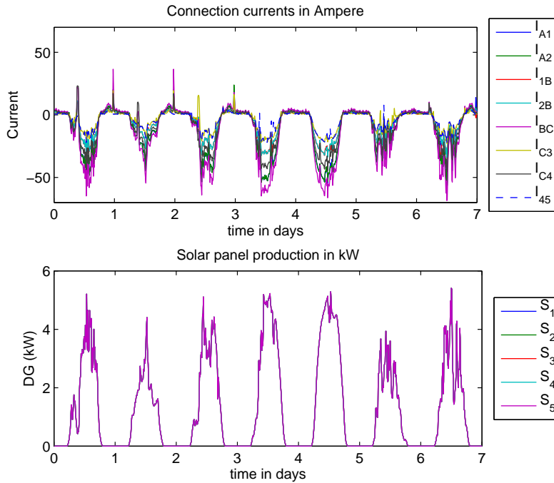
FIG. 5.2. Optimal ‘fair play’ configuration of solar panels: (top) current flow through each network edge for this configuration; (bottom) total solar generation at each household node is equal.
