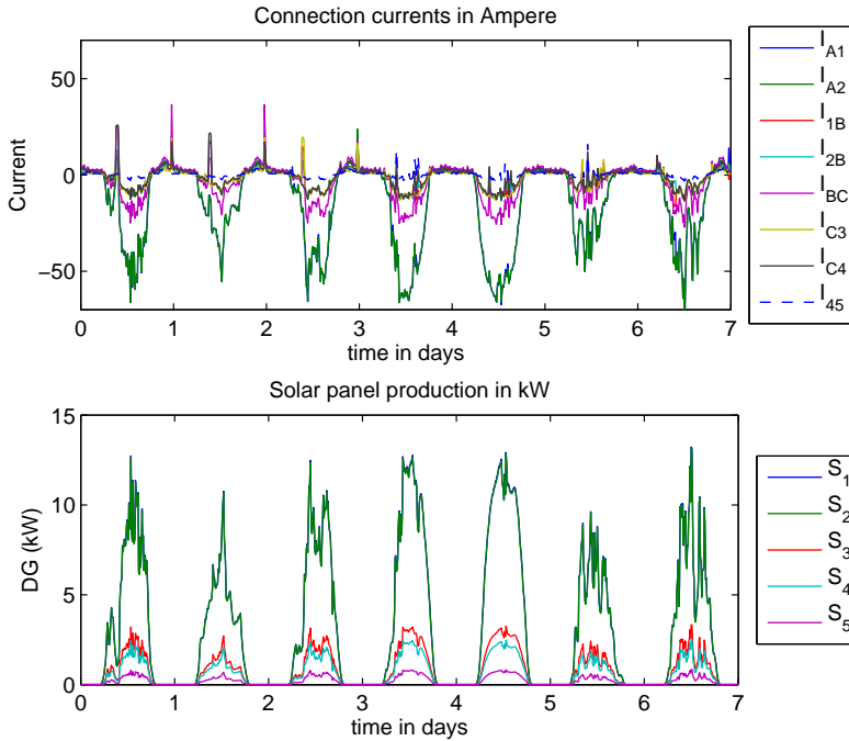
FIG. 5.1. Optimal configuration of solar panels: (top) current flow through each network edge for the optimal configuration (negative flow is upstream, consistent with a net surplus in decentral generation); (bottom) total solar generation at each household node for the optimal configuration.
