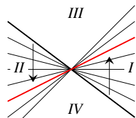
4) antipodal identification
