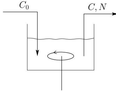
Figure 4.21: A chemostat.
