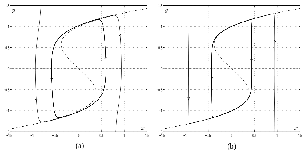
Figure 4.22: Phase portraits of (4.45): (a) \varepsilon = 0.1 ; (b) \varepsilon = 0.01 .
