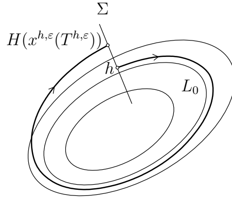
Figure 4.19: A segment \Sigma orthogonal to L_0 , together with unperturbed and perturbed orbits.
