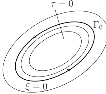
Figure 4.6: Normal coordinates near the cycle \Gamma_0 .
