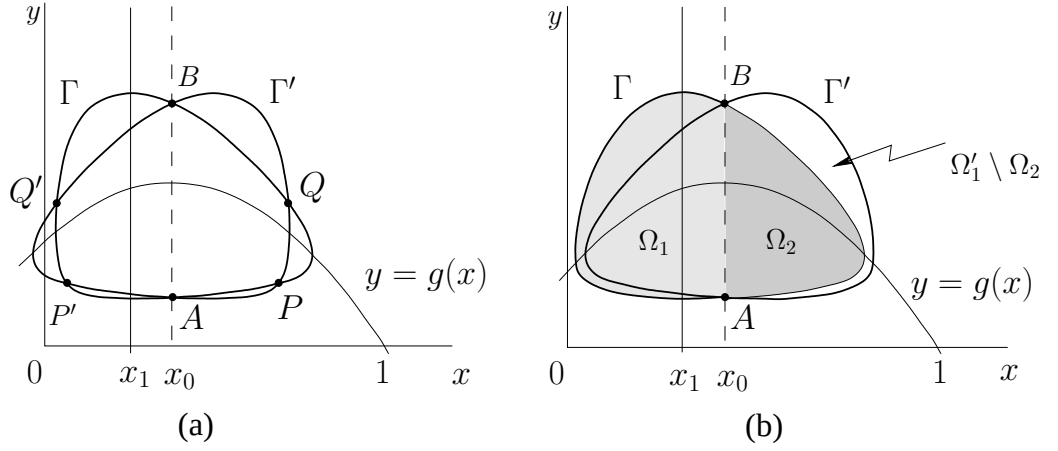
Figure 4.15: Geometry of the limit cycle: (a) real; (b) hypothetical.
