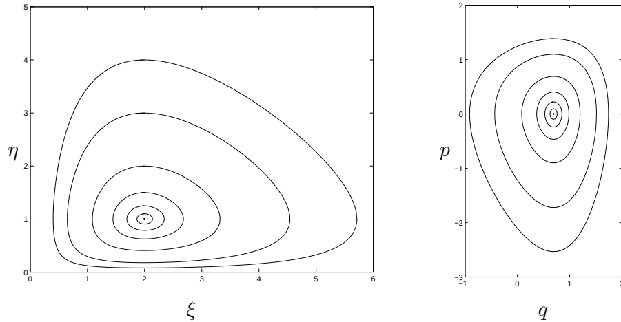
Figure 4.17: Phase portraits of the Lotka-Volterra system in the (\xi, \eta) - and (q, p) -coordinates.
