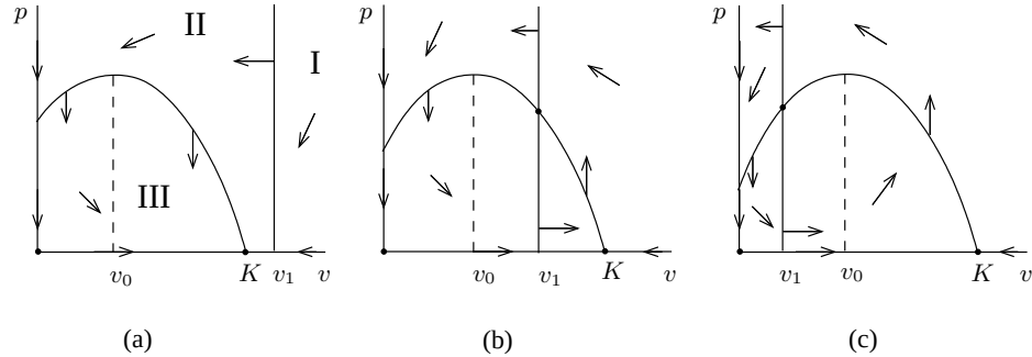
Figure 4.13: Zero-isoclines of (4.20).
