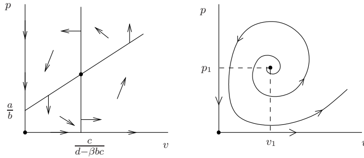
Figure 4.11: Zero-isoclines and the phase portrait of the system (4.16).
