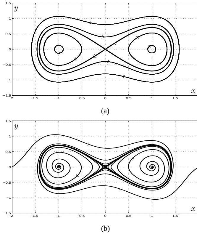
Figure 4.25: Phase orbits of (4.48): (a) \mu = 0 ; (b) \mu = -0.5 .
