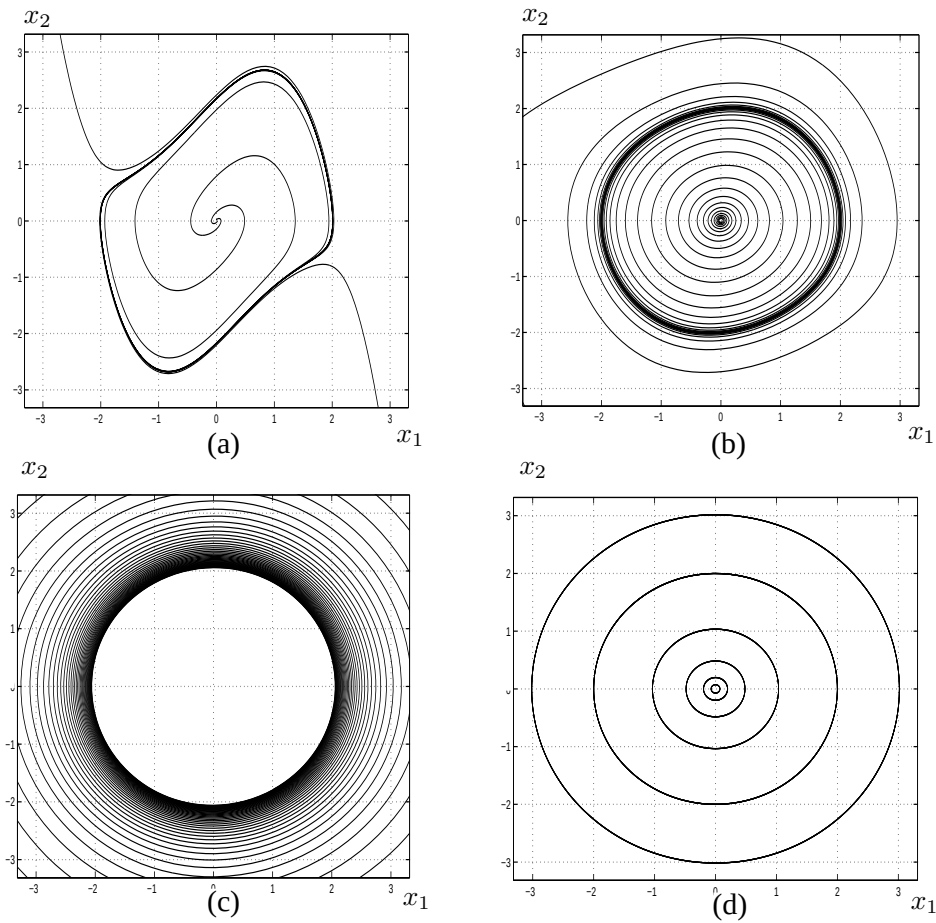
Figure 4.20: Phase portraits of Van der Pol equation: (a) \varepsilon = 1 ; (b) \varepsilon = 0.1 ; (c) \varepsilon = 0.01 ; (d) \varepsilon = 0 .
