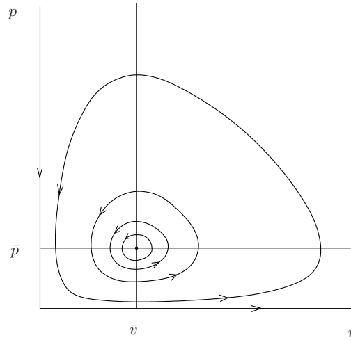
Figure 4.8: Phase portrait of the Lotka-Volterra system.
