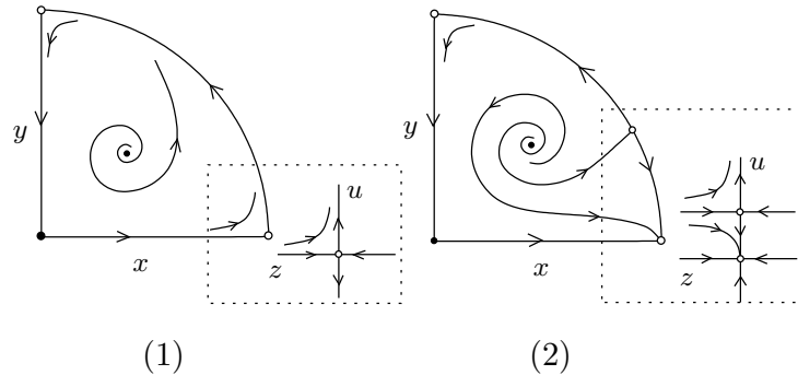
Figure 4.12: Behaviour of the system (4.16) at the infinity: (1) (d - \beta bc) - \beta ab \geq 0 ; (2) (d - \beta bc) - \beta ab < 0 .
