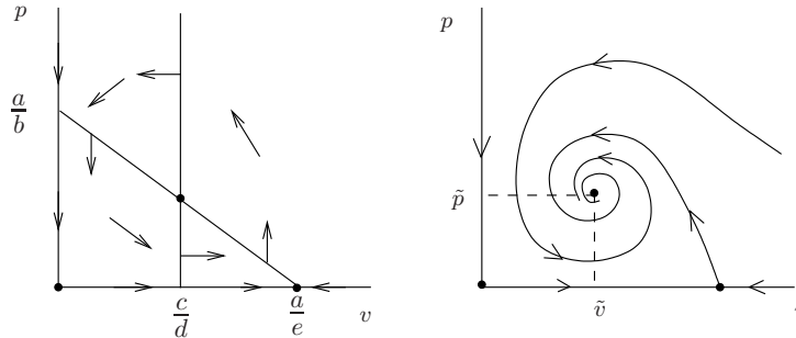
Figure 4.10: Zero-isoclines and the phase portrait of (4.13): ad - ce > 0 .
