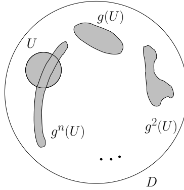
Figure 4.27: The recurrence phenomenon
