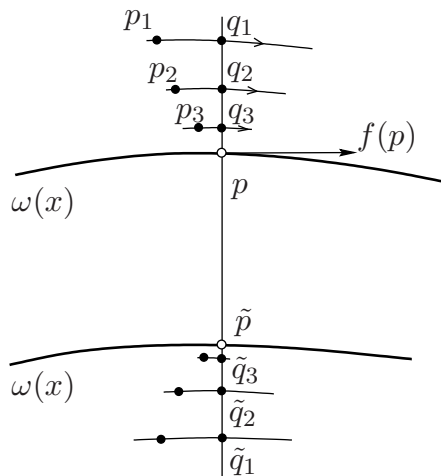
Figure 4.4: L \cap \omega(x) consists of only one point p .
