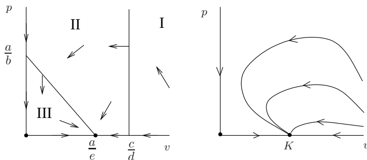
Figure 4.9: Zero-isoclines and the phase portrait of (4.13): ad - ce < 0 .
