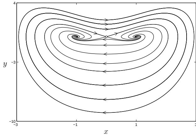
Figure 4.26: Phase portrait of a reversible system.
