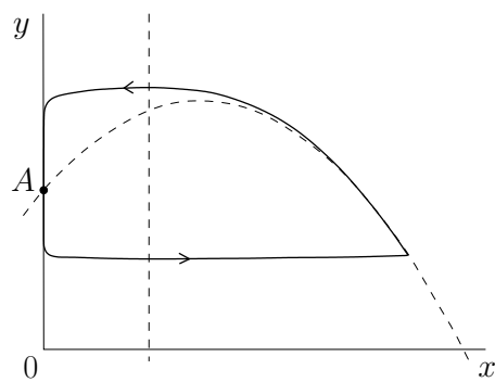
Figure 4.23: A slow-fast limit cycle in (4.46).
