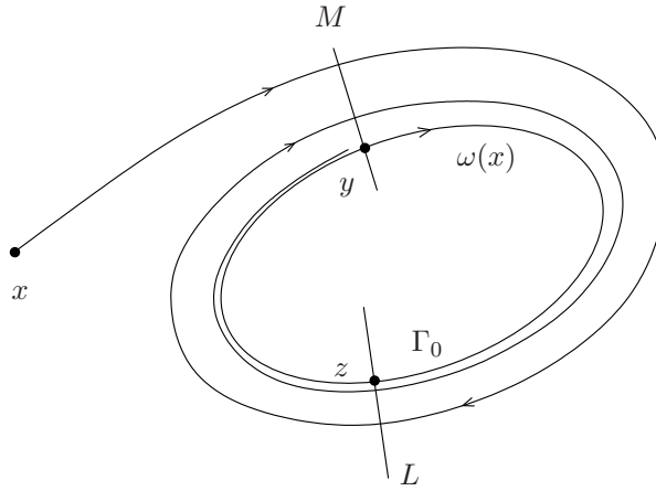
Figure 4.5: Lemmas 4.11 and 4.12.
