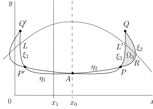
Figure 4.16: Geometrical constructions for the proof of uniqueness.
