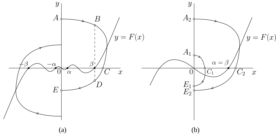
Figure 4.24: Analysis of limit cycles in Liénard system.
