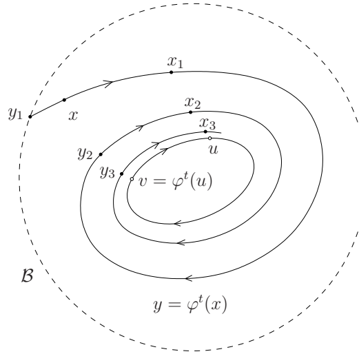
Figure 4.2: Backward invariance of \omega(x) .
