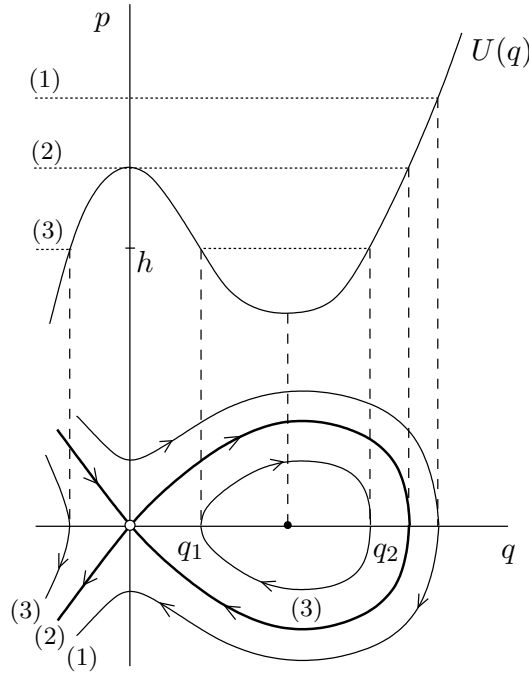
Figure 4.18: Newton dynamics with one degree of freedom.
