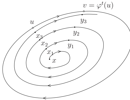
Figure 4.1: Forward invariance of \omega(x) .
