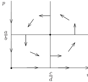
Figure 4.7: Zero-isoclines of the Lotka-Volterra system (4.10)
