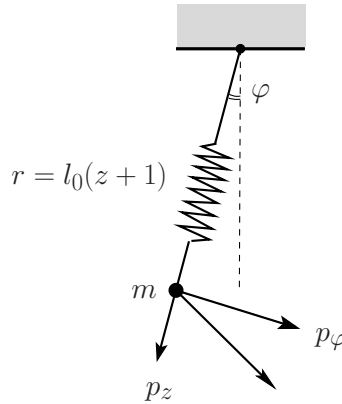
Figure 4.28: Elastic pendulum.
