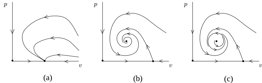
Figure 4.14: Generic phase portraits of the Rosenzweig-MacArthur system (4.20).
