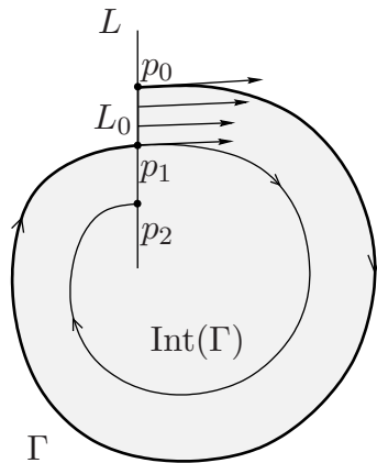
Figure 4.3: Monotonicity of the intersections.
