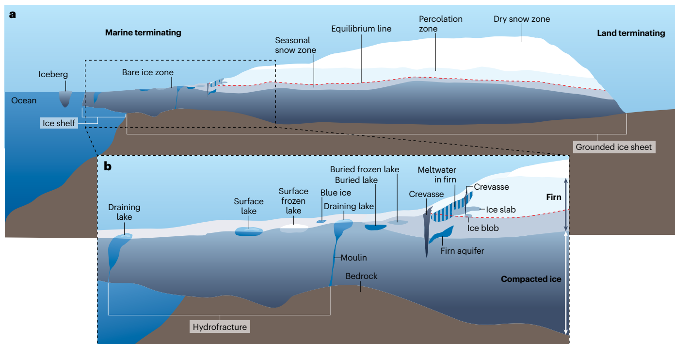
Fig. 1 | Schematic representation of important ice-sheet features. a, b , Full ice sheet (a) and a zoom in showing surface and hydrological features (b), including liquid water (blue), ice features (grey), crevasses (black) and bedrock under the ice (brown). Large parts of the Antarctic ice sheet terminate in ice shelves (left-hand side of panel a) whereas most of the ice sheet on Greenland terminates over land (right-hand side of panel a). The equilibrium line (red dashed line) separates the
