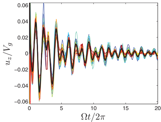
FIG. 2. (Color online) Times series of the vertical velocity u_z(x_0, z_0, t) measured at the center of the flow ( x_0=300 mm, z_0=240 mm), for 20 realizations performed at \Omega=0.84 rad s^{-1} (in various colors). The black thick line shows the ensemble average of these time series.
