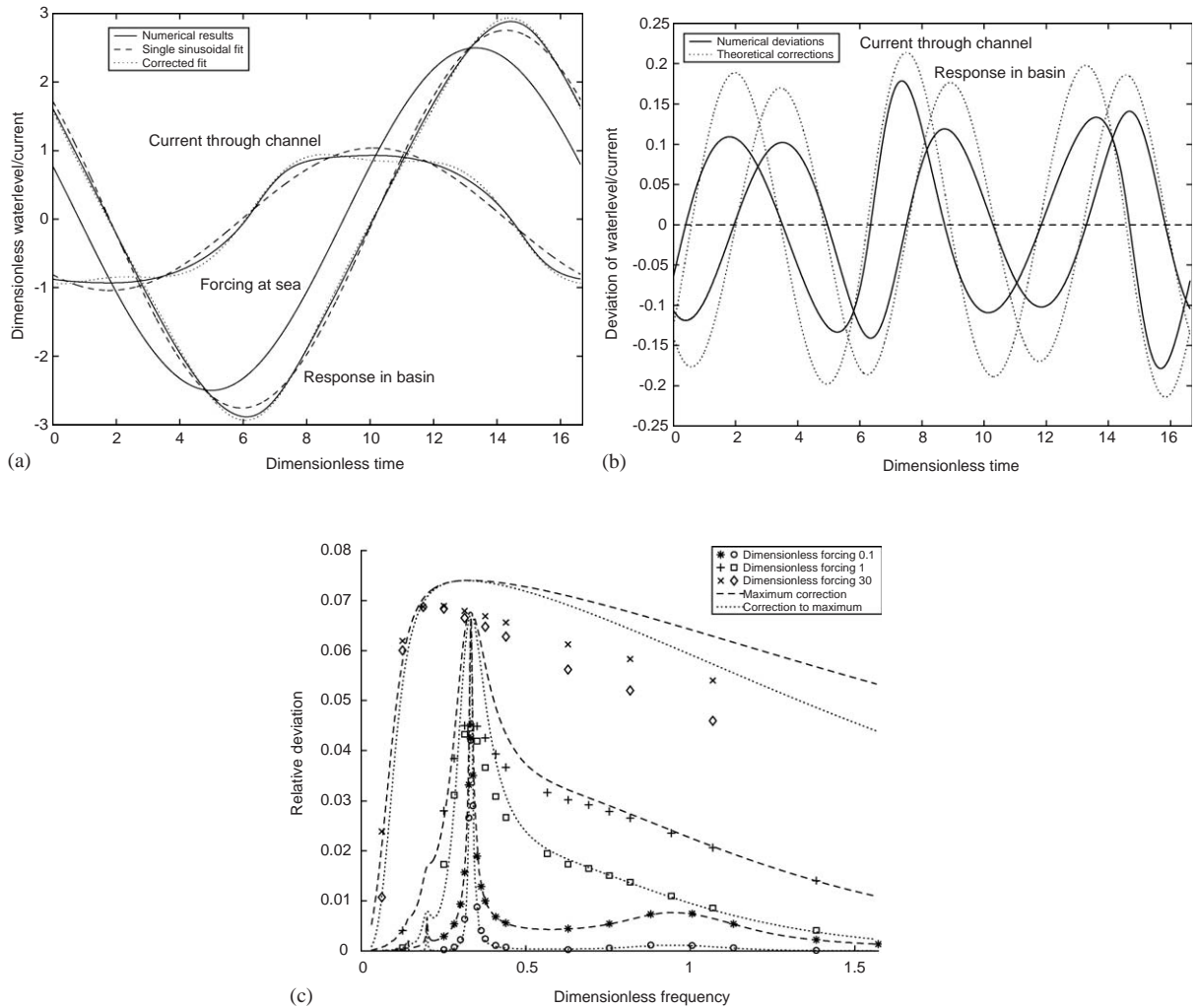
Fig. 6. Numerical results integrating (6) versus theoretical corrections using (10): (a) shows a sample tidal curve for \alpha'_e = 2.5 , \omega' = 0.377 . In (b) the dominant signal at the forcing frequency is subtracted. The maximum deviation from this signal (the maximum of the basin's water-level response in (b), asterisks, pluses and crosses) is plotted as a function of forcing frequency \omega' in (c), as well as the deviation of the maxima (high tide in (a), circles, squares and diamonds) from the single sinusoid's amplitude predicted by Lorentz' linearization theory, both relative to the amplitude of the single sinusoid. Results are obtained by numerical integration using DsTool for \alpha'_e = 0.1, 1 and 30 . The dashed lines approximate the maximum deviation, the dotted ones the deviation of the maxima, according to (10). The peak at \omega' = \frac{1}{3} is predicted well, although the amplitude is overestimated.
