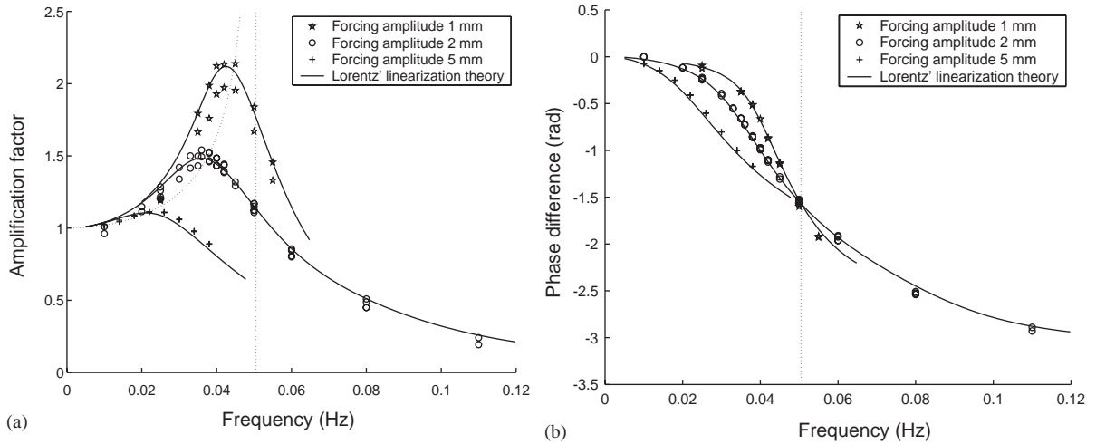
Fig. 4. Response curves: (a) amplification factor |\alpha|/\alpha_e and (b) phase lag \phi between the tide at sea and in the basin as a function of forcing frequency \omega/(2\pi) . Three series of measurements with forcing amplitudes \alpha_e \approx 1, 2, 5 mm are shown, for each of which results for two sensors in the basin have been obtained. Slight amplitude differences between both basin sensors can be noted, in particular at 1 mm forcing amplitude. Solid curves show the fit to theory (3). The Helmholtz frequency \omega_0 = 0.0505 Hz is indicated by a dotted vertical line, a dotted curve connects the maxima according to (4). Note that one fit is used to describe all three curves. Apparently the decrease of the resonator's quality is adequately described by Lorentz' linearization theory.
