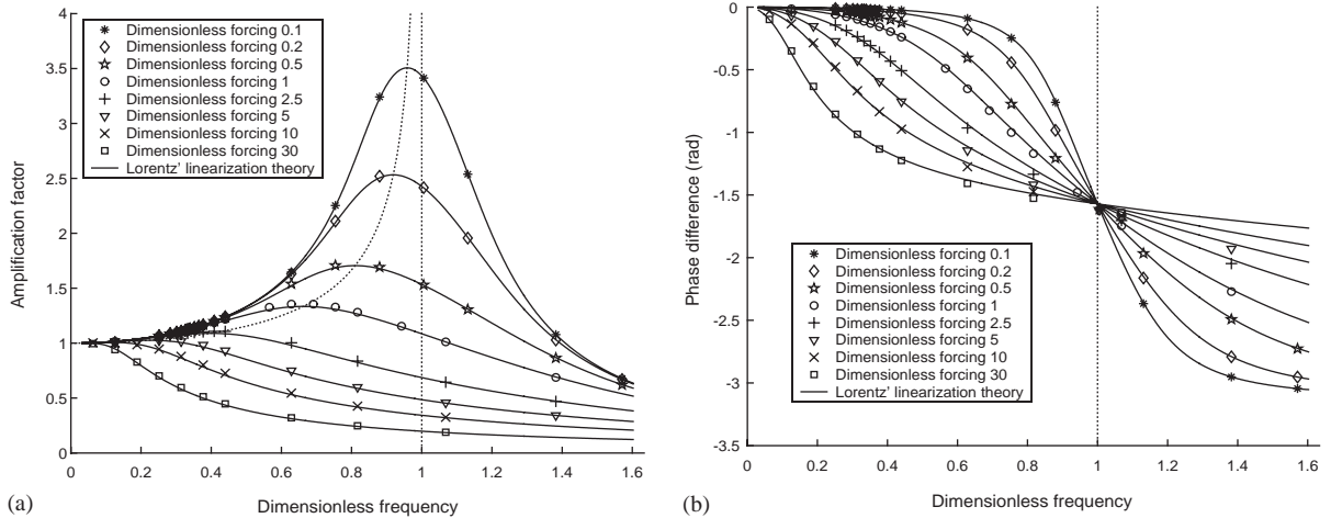
Fig. 5. Response curves: (a) amplification factor and (b) phase lag between the tide at sea and in the basin as a function of forcing frequency. Numerical results (symbols) for the dimensionless system (6) are shown. The dimensionless Helmholtz frequency \omega'_0 = 1 is indicated by a dotted vertical line, a dotted curve connects the maxima according to (4). The theoretical (solid) curves are calculated from (3),(4), with \omega_0 = 1 , \nu_0 = 8/3\pi .
