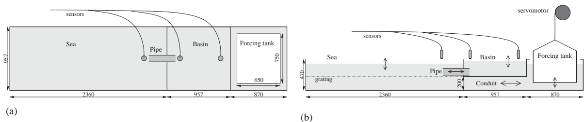
Fig. 2. Sketch of the experimental setup, dimensions in mm are indicated. The forcing tank is set into motion by a servomotor. The water expelled by the tank moves through the conduit underneath the basin area to the “sea”. The tidal signal thus generated at sea, propagates into the basin through a completely submerged pipe. The water-level elevation is measured by acoustic sensors at the indicated positions. Because the tide in the basin is nearly uniform, the measurements for the sensors in the basin are virtually the same. (a) Top view, (b) side view.
