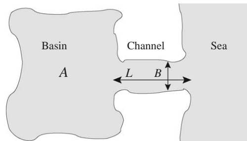
Fig. 1. Top view sketch of an almost-enclosed tidal basin with horizontal area A , co-oscillating with the tide at sea through an inlet channel of width B , length L and depth H .
