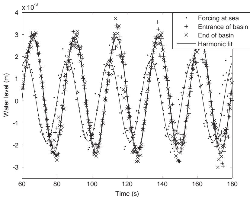
Fig. 3. Sample time series of measurements at forcing frequency 0.0420 Hz and forcing amplitude approximately 2 mm. Dots indicate measurements from the sensor at sea, pluses and crosses indicate measurements at the entrance and end of the basin, respectively. Solid curves show harmonic fits to the respective time series. The two curves inside the basin are nearly indistinguishable, consistent with a Helmholtz mode of uniform basin tide.
