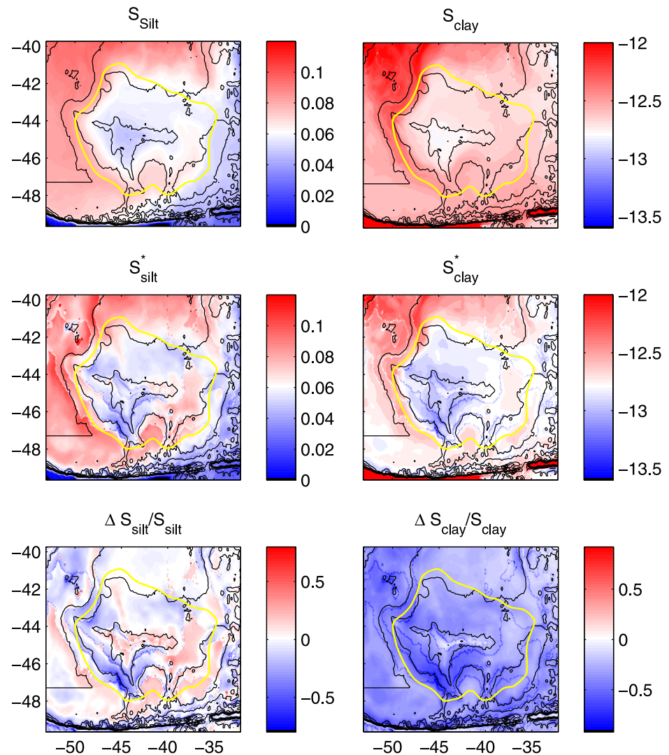
Figure 12. Sedimentation rates for silt (left; \text{Mgm}^{-2}\text{s}^{-1} ) and clay (right; log-scale) in the ZR region. Shown are averages over years 5 and 6 of the standard simulation (top), and the branch simulation with modified sedimentation formulation (middle). Figure 12 (bottom) show the fractional difference between these fields, with \Delta S = S^* - S .
