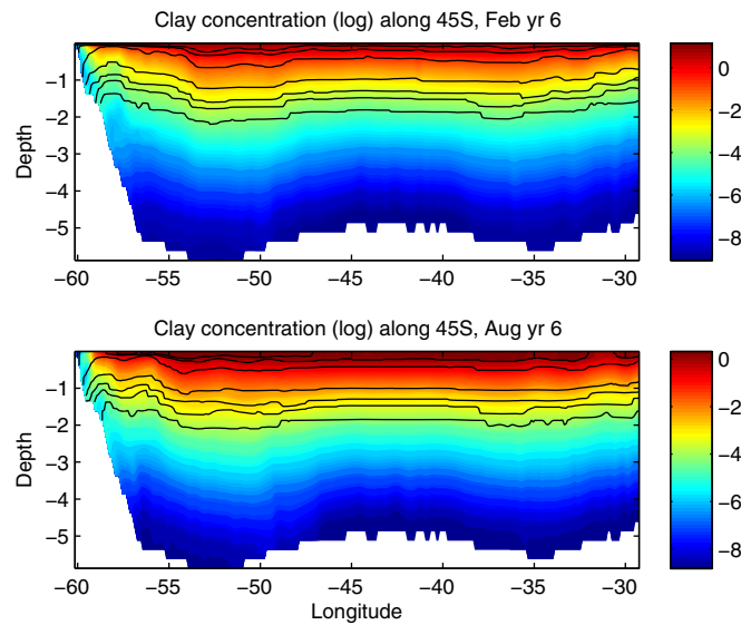
Figure 7. Distribution of the clay fraction ( \log(C_{clay}) ) along 45^\circ\text{S} across the Zapiola Rise. Monthly averages for February (top) and August (bottom) of year 6 of the simulation. Contours are select isopycnals.
