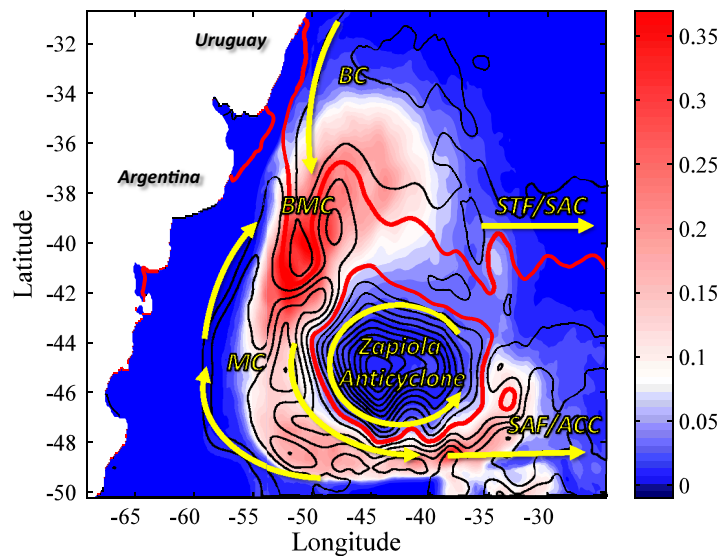
Figure 2. Vertically integrated eddy kinetic energy per unit area (shading; 10^6\text{kgs}^{-2} ); and distribution of barotropic stream function (contours; interval 25 Sv, zero-contour in red), as represented by the POP model. Arrows schematically indicate the major flow features, in particular the Zapiola Anticyclone; the Malvinas Current (MC), Brazil Current (BC), and their confluence (BMC); the South Atlantic Current (SAC) and the associated Subtropical Front (STF); and the continuation of the Antarctic Circumpolar Current (ACC) along the Subantarctic Front (SAF).
