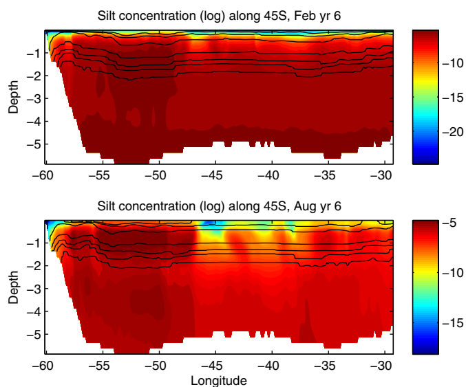
Figure 6. Distribution of the silt fraction ( \log(C_{silt}) ), along 45^{\circ}\text{S} across the Zapiola Rise. Monthly averages for February (top) and August (bottom) of year 6 of the simulation. Contours are select isopycnals.
