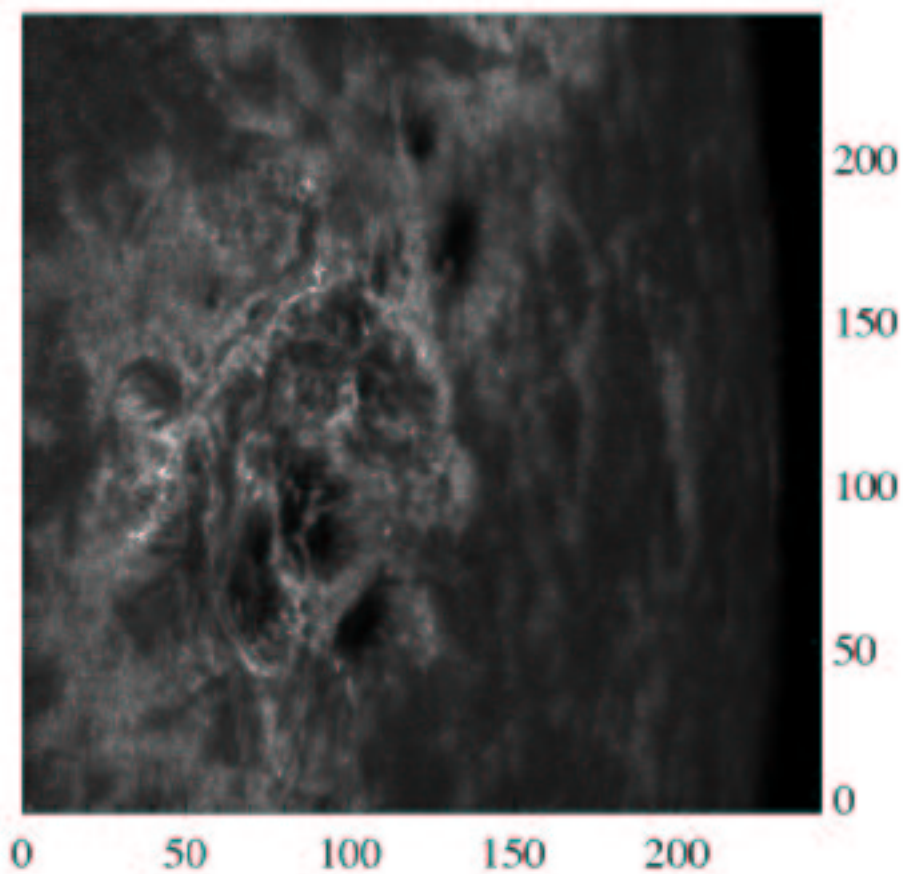
Ca II H (397nm)
