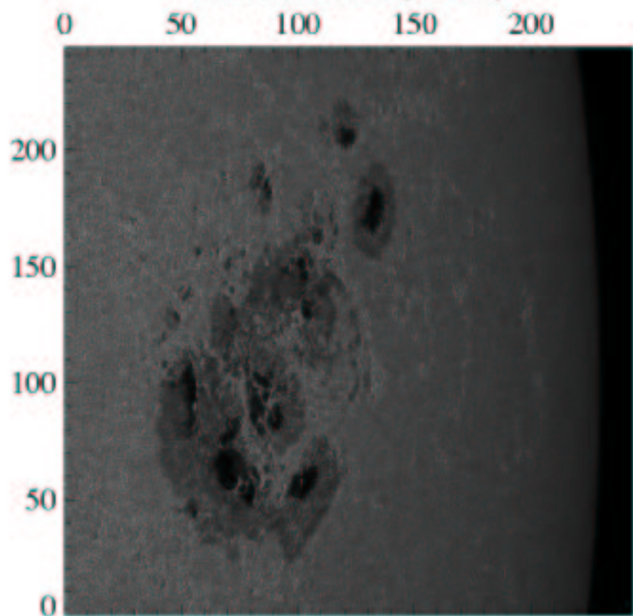
Blue continuum (432nm)
