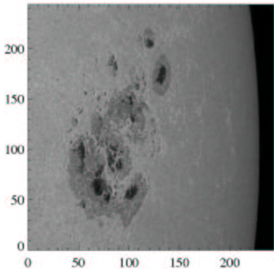
Red continuum (656nm)
