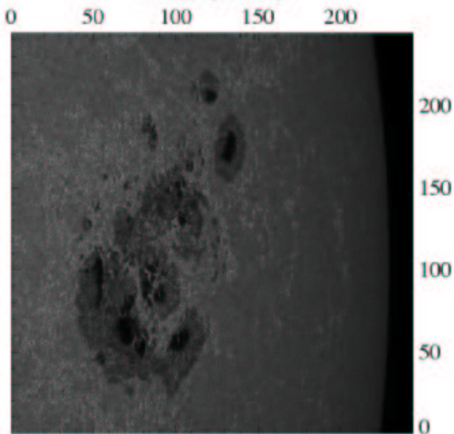
G band (430nm)
