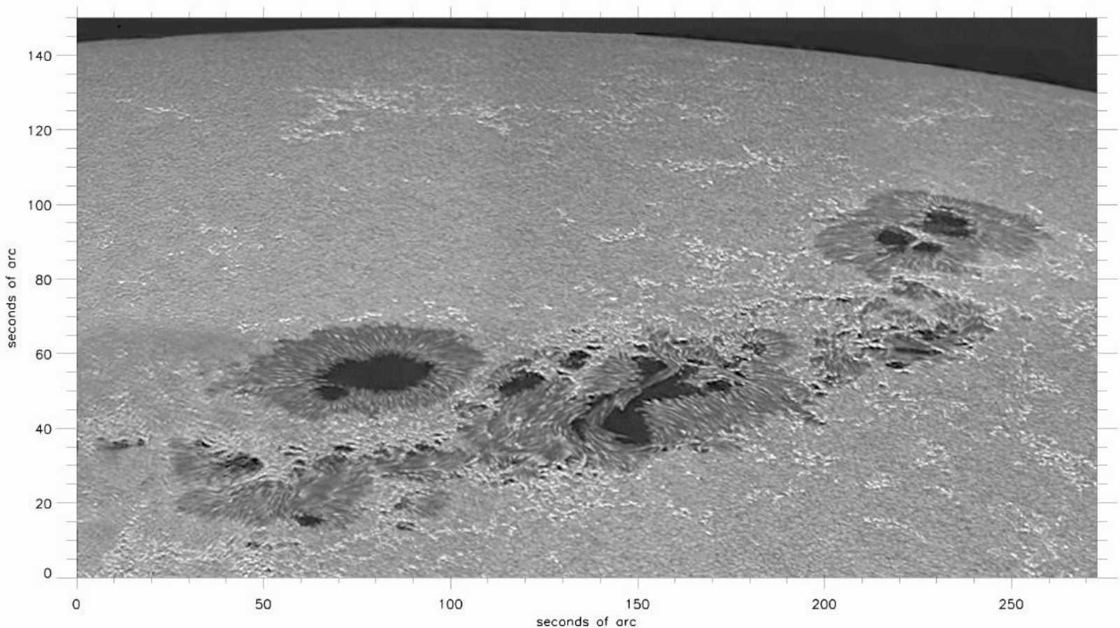
AR 9393 on April 1, 2001
