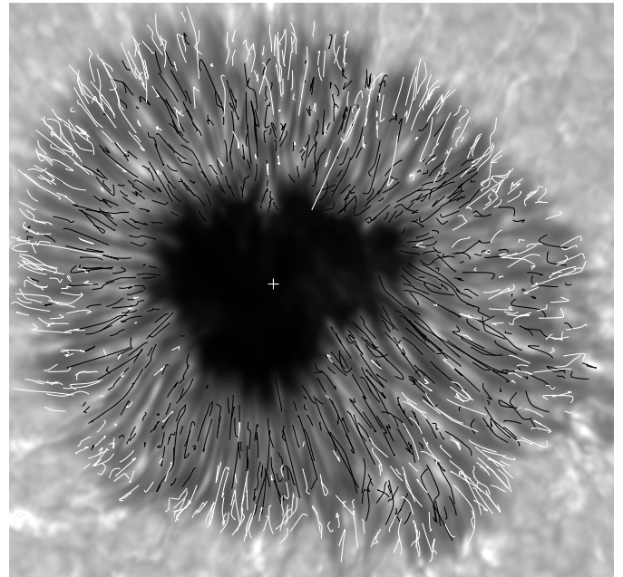
Fig. 3. Trajectories of INW (black) and OUT (white) PGs. The underlying image is an average of all frames in the series. The center of the umbra is marked by a white cross. The image size is 29.8 \times 28.4 Mm.
