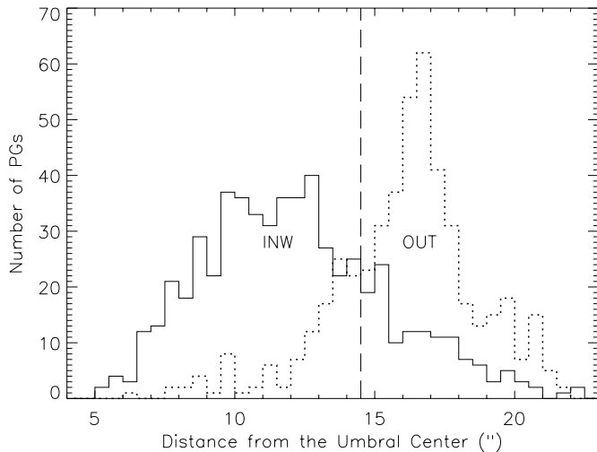
Fig. 2. Histogram of time-averaged distances of the INW (solid line) and OUT (dotted line) PGs from the center of the umbra. The position of the dividing line is marked by vertical dashes.
