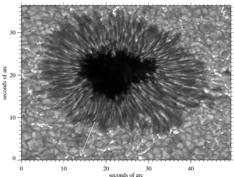
Fig. 1. A speckle reconstructed image of sunspot NOAA 8704. The arrow marks the direction towards disk center.
