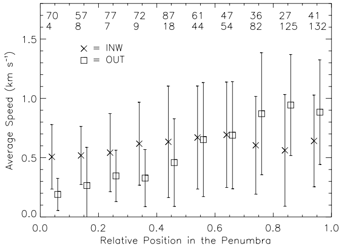
Fig. 4. Average speed of PGs as a function of their relative positions in the penumbra. INW PGs are represented by \times , OUT PGs by \square . Position 0.0 is at umbra, 1.0 at photosphere. The bars indicate a scatter of \pm 1\sigma . Numbers of INW (OUT) PGs in each bin are displayed in the upper (lower) row.
