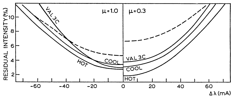
Figure 3. Computed ( solid ) and observed ( dashed ) line cores of the Na D_1 line. Viewing angles \mu = 1.0 (left) and \mu = 0.3 (right).
