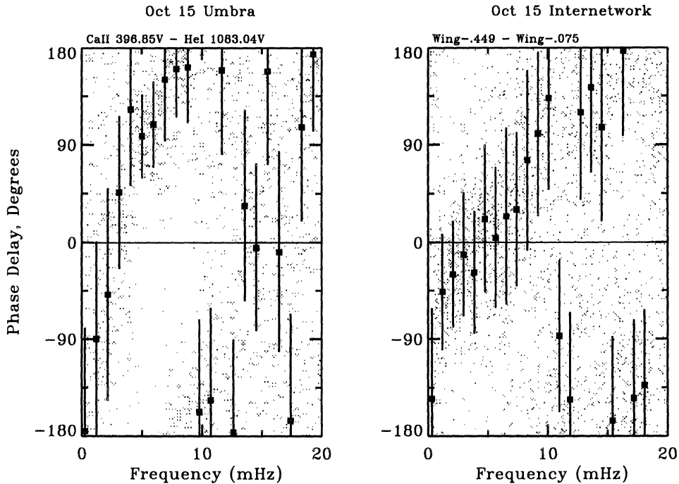
Fig. 5. Left: V - V phase differences between H_3 Doppler shift and He I 1083.0 Doppler Shift for an umbra. Right: I - I phase differences between the intensities at \Delta\lambda = -0.449 nm and -0.075 nm from H_3 , for the quiet Sun internetwork pixels at the far right in Fig. 1.
