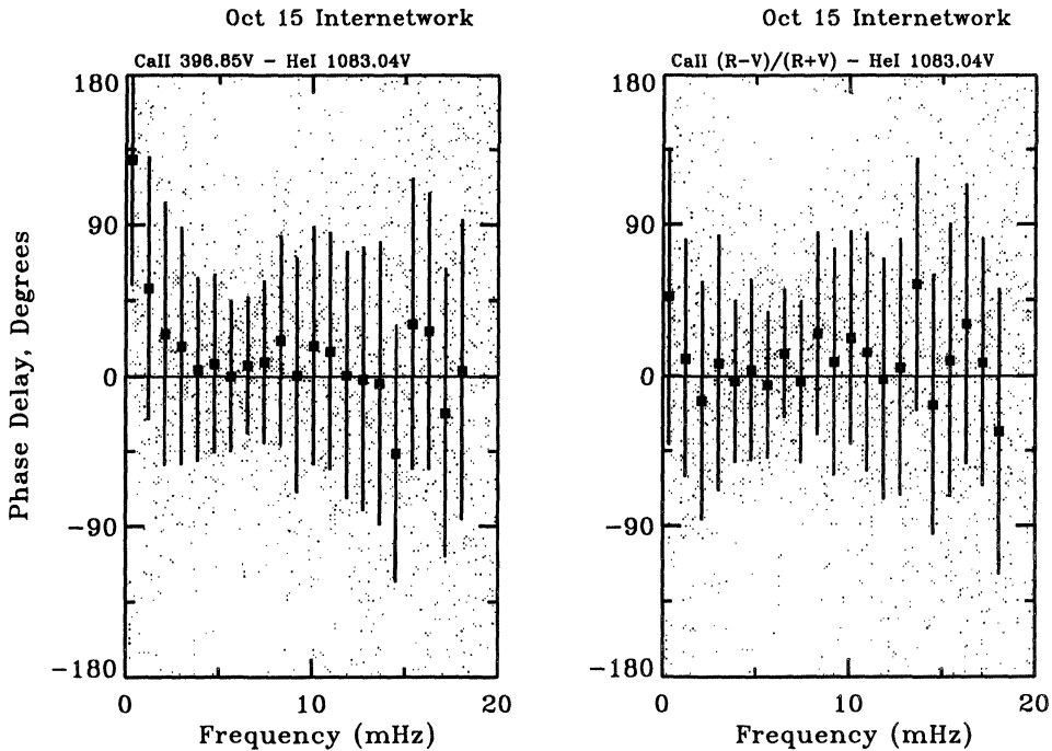
Fig. 4. Phase difference spectra for the quiet Sun internetwork at the far right in Fig. 1, respectively between H 3 Doppler shift and He I 1083.0 Doppler shift (left) and between the Ca II H (R - V)/(R + V) ratio and He I 1083.0 Doppler shift (right).
