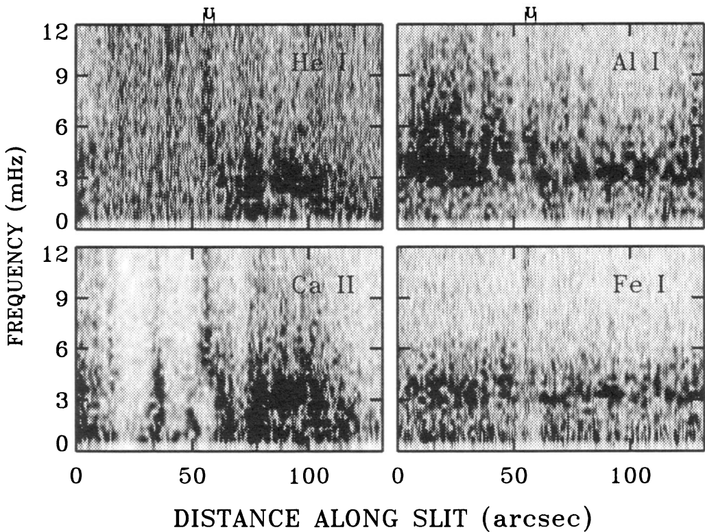
Fig. 2. Power spectra as in Fig. 1 for an area containing a small pore (marked by the symbols U at the top).
