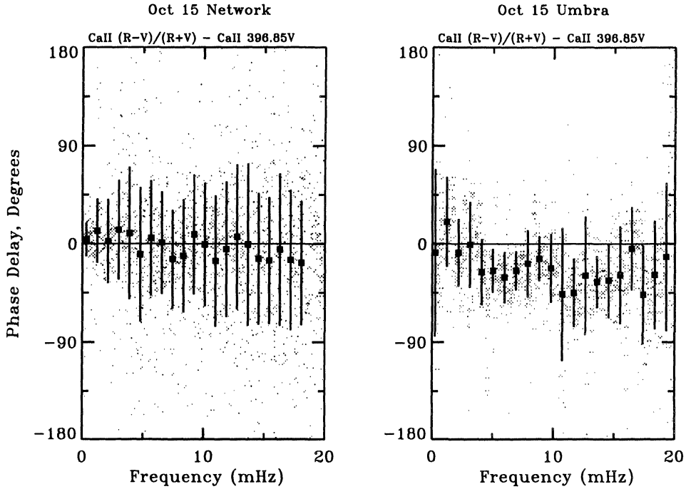
Fig. 3. Phase difference spectra between the Ca II H (R - V)/(R + V) ratio and H 3 Doppler shift. Left: network. Right: umbra. The scattered points are independent determinations from different spatial positions. The bars are 1\sigma deviations from their averages (squares) per frequency bin.
