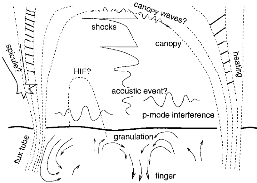
Figure 5. Cartoon of the structure of the lower solar atmosphere outside active regions. See also Fig. 2 of the review by Judge and Peter (1998). It shows, schematically, various phenomena in a vertical cut through the lower atmosphere, and covers about the same radial domain as portrayed in Fig. 2. The magnetic network (dashed fieldlines) is thought to be made up of thin 1400 Gauss fluxtubes that are best seen in the 430.5 nm G band (Title and Berger, 1996; magnificent Scharmer-Berger poster available at http://diapason.lmsal.com/~berger/ ). They tend to be embedded in fast downflows that occasionally cause upward propagating shocks (Steiner et al. , 1998) that seem most likely to cause the overly ignored spicules (Beckers, 1968). Higher up, the field is expected to expand and form a low-lying magnetic canopy when it connects with neighboring network field (e.g., Giovanelli and Jones, 1982; Jones and Giovanelli, 1983; Solanki and Steiner, 1990; Bruls and Solanki, 1995; Briand and Solanki, 1995). The magnetic heating, whatever way it is done, does apparently not expand with the field since the network remains sharply grained in ultraviolet images diagnosing much higher temperatures than sketched here. The enclosed internetwork volume is free of kilogauss fields but does contain isolated patches of 500 Gauss field that may consist of weaker fluxtubes (Lin, 1995; Solanki et al. , 1996), isolated patches of weaker horizontal field (Litee et al. , 1996) which are perhaps a subclass of field structures with all sorts of inclinations (Meunier et al. , 1998), and possibly a truly weak diffuse field. The main structuring in the deep photosphere is the shallow granulation pancake pattern caused by radiative losses from convective upwellings. Deep downflow fingers marked by long-lived "intergranular holes" may produce "acoustic events" (Restaino et al. , 1993; Rimmele et al. , 1995; Roudier et al. , 1997; Hoekzema et al. , 1998a) in the middle photosphere, which is otherwise dominated by the 5-minute oscillation, the interference pattern of the multitude of solar p -modes. Higher up the higher-frequency components gain dominance and contribute to the K_{2V} -grain producing acoustic shocks (Rutten and Uitenbroek, 1991; Carlsson and Stein, 1997). These have also been diagnosed in rocket spectrograms (Hoekzema et al. , 1997) and are now seen very well, again as bright internetwork grains, in the TRACE 160 nm images at http://vestige.lmsal.com/TRACE/Public/FirstLight/ . The occurrence of the brightest of these shock-produced internetwork grains is here attributed to pistoning by strong subsurface downflows; if so, the TRACE 160 nm image sequences may provide input piston sites for local helioseismology (Duvall et al. , 1993). The shocks may also excite canopy waves (Hoekzema et al. , 1997) that may funnel down into the network tubes (Deubner and Fleck, 1990) and may have to do with the FIP fractionation (Rutten, 1997). Scales: fluxtube diameters 0.1–0.2", granule diameters 0.5–1.5", five-minute oscillation patches 5–15", three-minute shock patches 1–3", internetwork cell sizes 20–40", canopy heights unknown.
