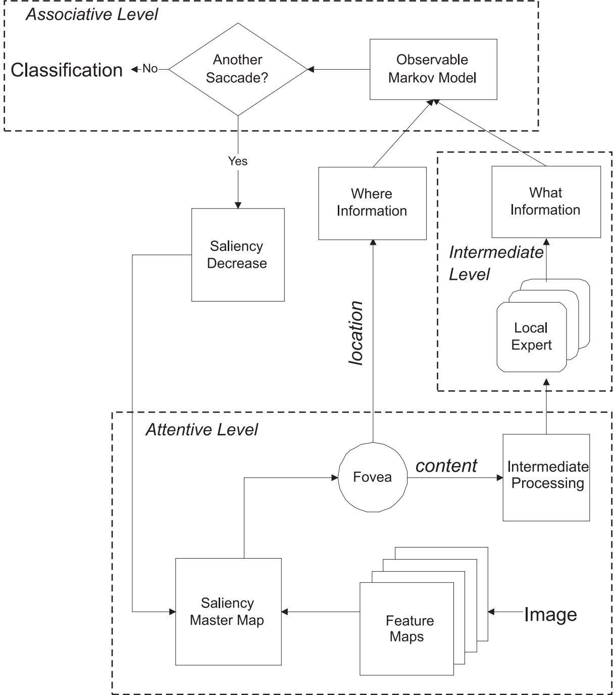
Figure 1. The selective attention model for visual recognition
