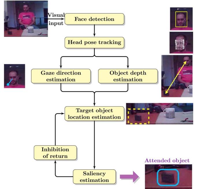
Fig. 2. Basic steps of the algorithm.
