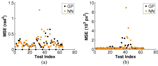
Fig. 13. MSEs for (a) gaze estimation (in terms of radian squared) and (b) object depth estimation (in terms of 10^3 pixel squared).
