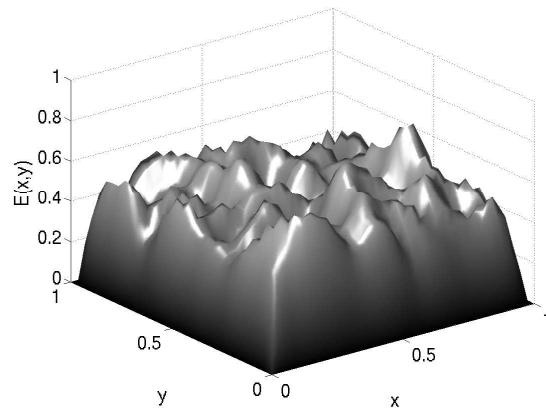
Error after 3 Jacobi iterations
