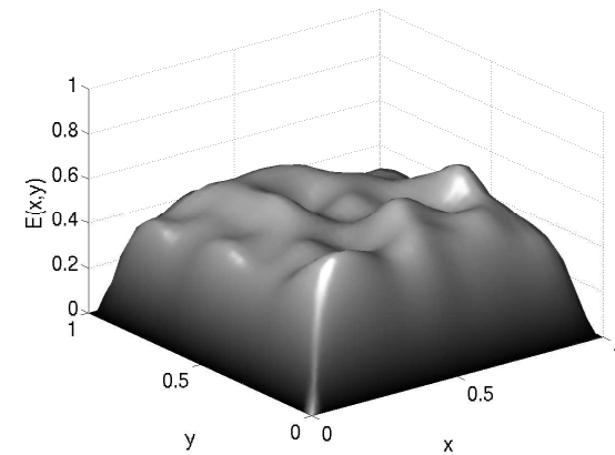
Error after 8 Jacobi iterations
