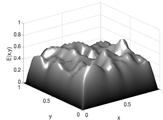
Error after 4 Jacobi iterations
