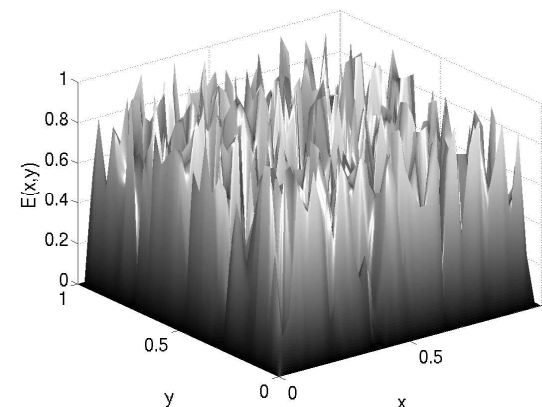
Random initial error
