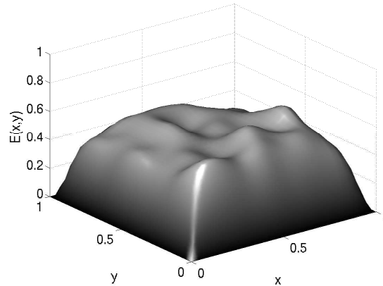
Error after 10 Jacobi iterations
