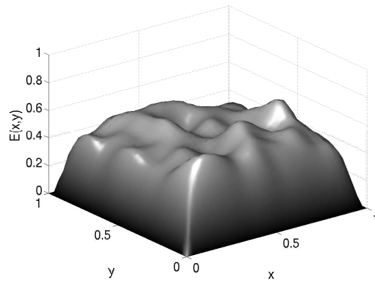
Error after 7 Jacobi iterations
