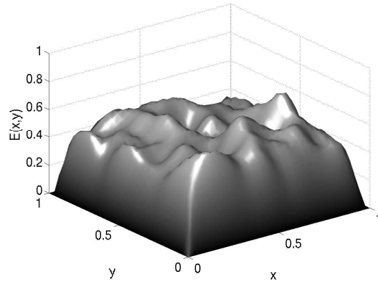
Error after 5 Jacobi iterations
