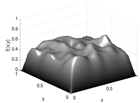
Error after 6 Jacobi iterations
