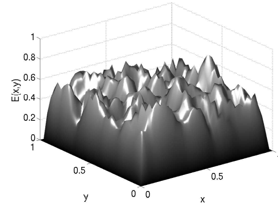
Error after 2 Jacobi iterations
