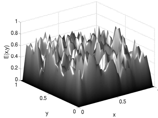
Error after 1 Jacobi iterations
