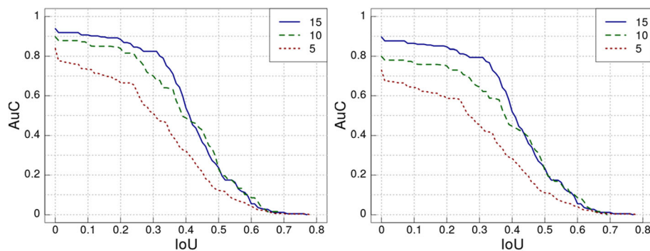
Fig. 9 Mean AuC over all interactions using four-fold cross-validation with different numbers of training sequences, for SC (left) and MC (right)
