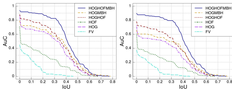
Fig. 7 Mean AuC over all interactions using four-fold cross-validation in the SC (left) and MC (right) scenarios of ShakeFive2
