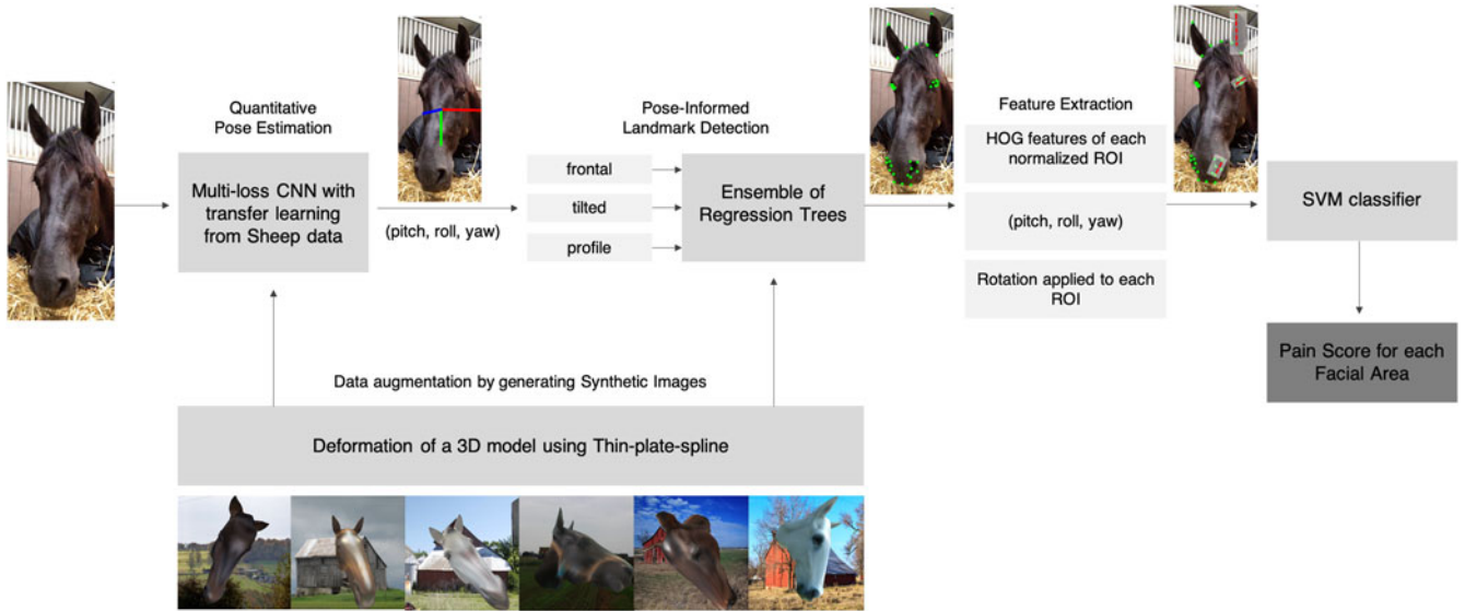
Fig. 4. Proposed pipeline for horse pain estimation based on facial features.
