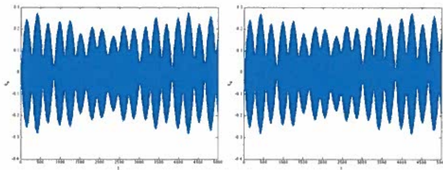
Fig. 9. Time series ([0, 5000]) of q_6(t) and q_8(t) starting with zero initial conditions. The parameter values are as in Figs. 7 and 8.
