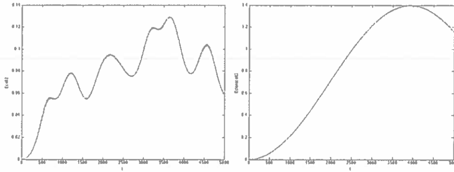
Fig. 3. Time series ([0, 5000]) of the energy of the second cell, left the 1: 2: 3 resonance (scale [0, 0.14] ), right the classical case (scale [0, 1.4] ). The link is linear and exists between q_2 and q_6 ; the initial conditions of the first cell start near the eigenmode x_1 and are given in Table 1, the second cell starts with zero energy; \varepsilon = 0.2, \mu = 0.1 .
