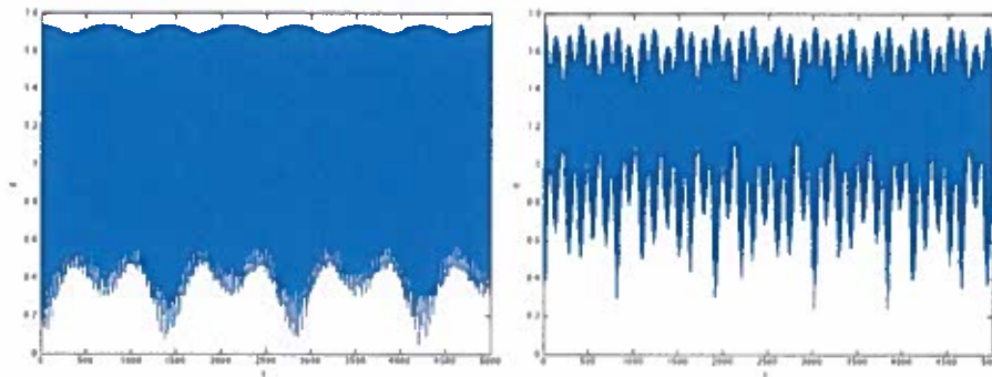
Fig. 7. Time series ([0, 5000]) of the Euclidean distance d starting near the x_2 eigenmode in the first classical FPU cell (left, scale [0, 1.8] ). For the initial conditions indicated in Table 1 the recurrence is quite good. On the right (scale [0, 1.8] ) the time series for two cells with the same initial conditions; the recurrence is delayed.
