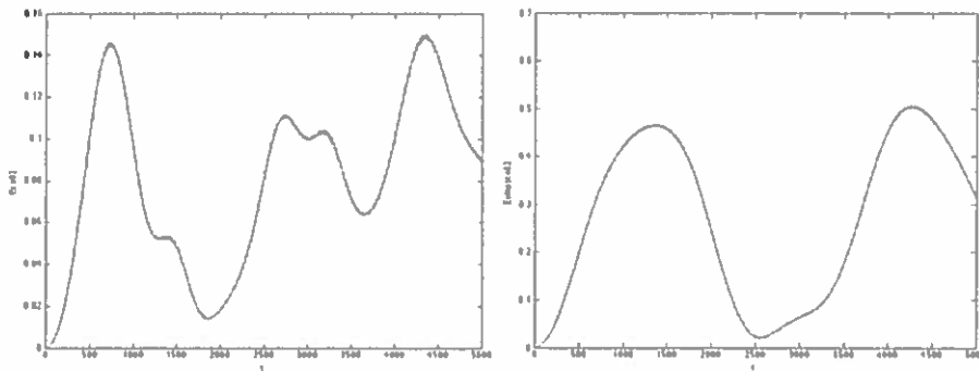
Fig. 4. Time series ([0, 5000]) of the energy of the second cell, left the 1: 2: 3 resonance (scale [0, 0.16] ), right the classical case (scale [0, 0.7] ). The link is linear and exists between q_2 and q_6 ; the initial conditions of the first cell start near the eigenmode x_2 and are given in Table 1, the second cell starts without energy; \varepsilon = 0.2, \mu = 0.1 .
