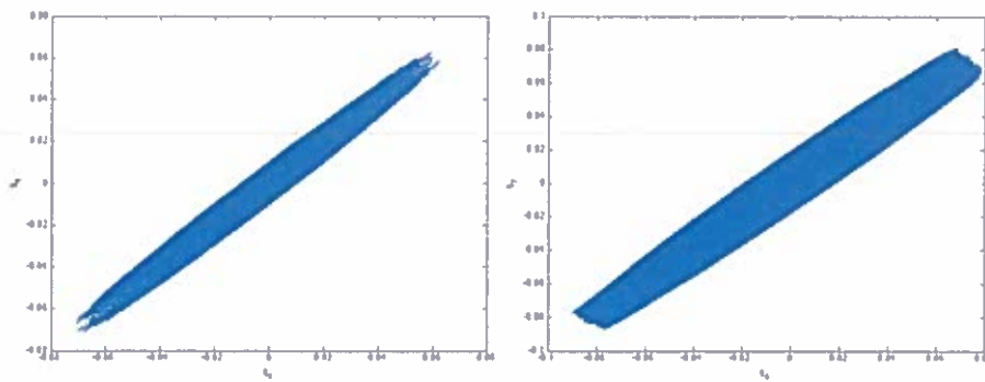
Fig. 8. Starting near the x_2 spectral normal mode of Table 1 in the first cell, mode 5 and 7 in the second cell are near to 1:1 resonance which is typical for the classical case. The q_5 - q_7 diagram left took 250 time steps, right 5000. The 1:1 resonance is very slowly destroyed, the recurrence in the system of two cells takes clearly more than 5000 time steps. Parameter values m = 0.1 , \varepsilon = 0.2 , \mu = 0.1 .
