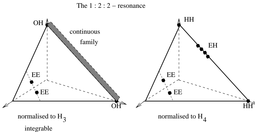
Figure 2: The three d-o-f (1 : 2 : 2)-Hamiltonian resonance, left the periodic solutions in an action simplex of the Hamiltonian normalised to H_3 , right normalization to H_4 (figure courtesy Springer).
