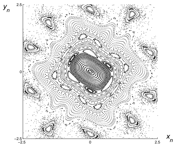
Figure 1: The area-preserving map T_H produced by eq. (1) for \alpha = 3\pi/5 . In the centre of the plane there is a dominant family of closed KAM-curves. In between the curves there are again stable and unstable periodic solutions but they can not be observed at this level of precision. Outside this family of closed curves one finds stable periodic solutions associated with unstable periodic solutions. Moving out one observes a stable and unstable 10-periodic solution and further on another pair of 10-periodic solutions. The unstable solutions have stable and unstable manifolds that intersect an infinite number of times producing chaotic behaviour. The dots correspond with orbits returning chaotically in the plane when applying the map repeatedly. Poincaré described the folding process, see [17], that can be seen dynamically by considering a small square in the plane and following its subsequent mappings (figure courtesy Igor Hoveijn).
