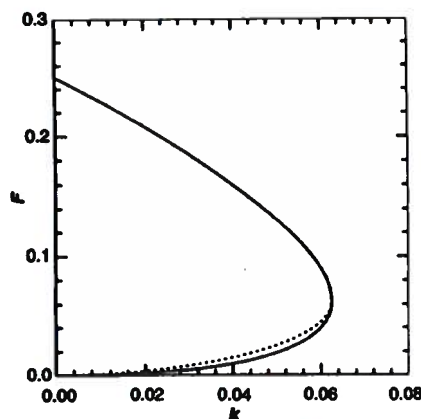
Fig. 1. Phase diagram of the reaction kinetics. Outside the region bounded by the solid line, there is a single spatially uniform state (called the trivial state) (U = 1, V = 0) that is stable for all (F, k) . Inside the region bounded by the solid line, there are three spatially uniform steady states. Above the dotted line and below the solid line, the system is bistable: There are two linearly stable steady states in this region. As F is decreased through the dotted line, the non-trivial stable steady state loses stability through Hopf bifurcation. The bifurcating periodic orbit is stable for k < 0.035 and unstable for k > 0.035 . No periodic orbits exist for parameter values outside the region bounded by the solid line.
