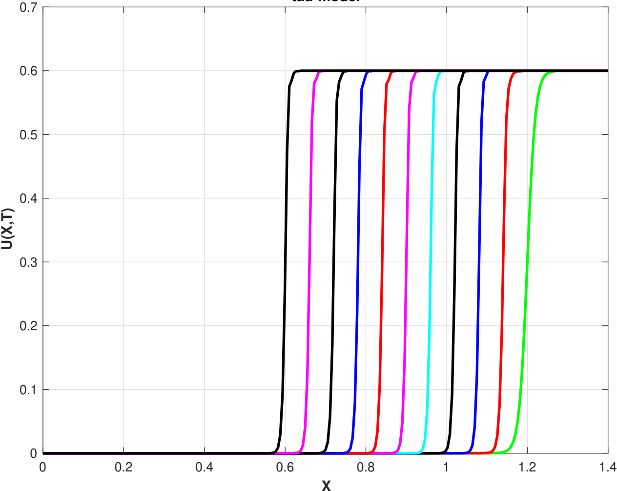
tau-model
