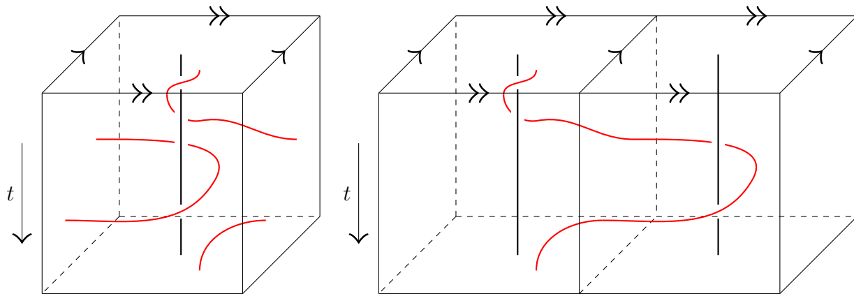
(a) A braid on the torus.
