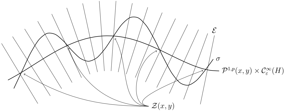
Figure 4: \mathcal{Z}(x, y) as transverse intersection of the section \sigma and the zero section \mathcal{P}^{1,p}(x, y) \times \mathcal{C}_\varepsilon^\infty(H) in the fiber bundle \mathcal{E} .
