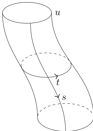
Figure 2: Schematic shape of a trajectory u .
