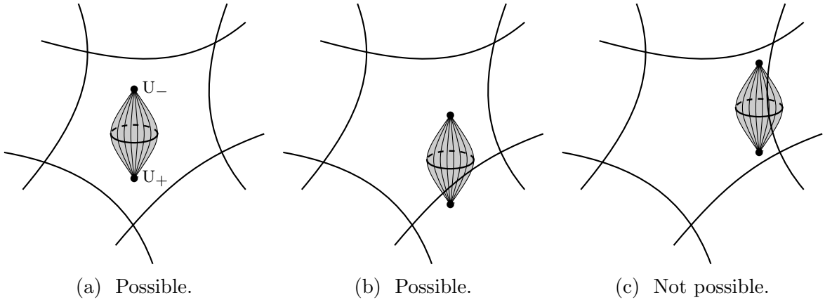
Figure 7: Proper braid class [X \text{ rel } Y] with examples of spaces \mathcal{M}(u_-, u_+) .
