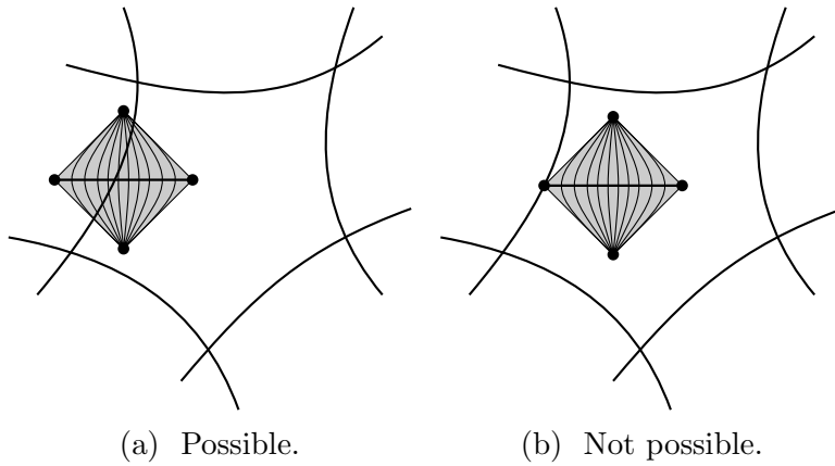
Figure 9: Proper braid class [X \text{ rel } Y] with even more examples of spaces \mathcal{M}(U_-, U_+) .
