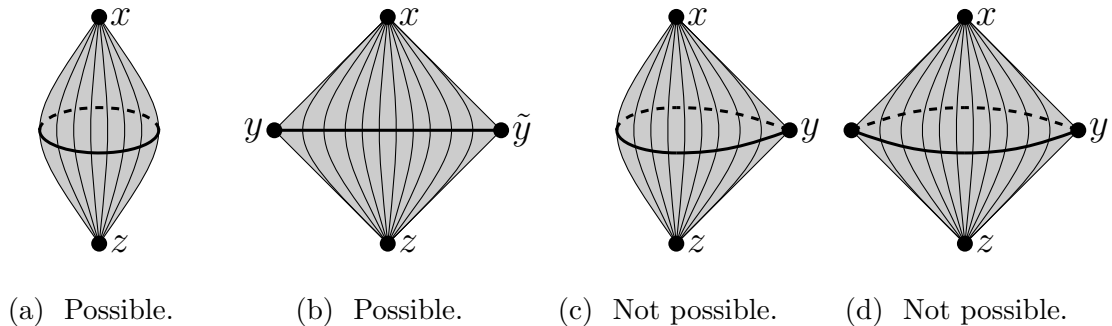
Figure 6: Example spaces \mathcal{M}(x, z) in grey with there broken trajectories. The thick line in the middle shows the corresponding trajectory spaces \mathcal{L}(x, z) .
