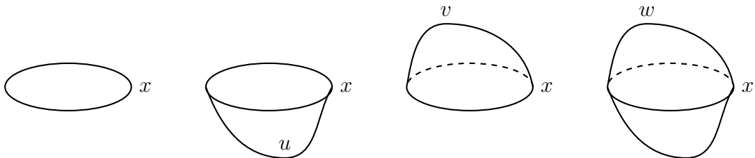
Figure 1: A contractible loop x [left] in M with its extensions u and v [middle]. The extensions u and v form together a sphere w [right].
