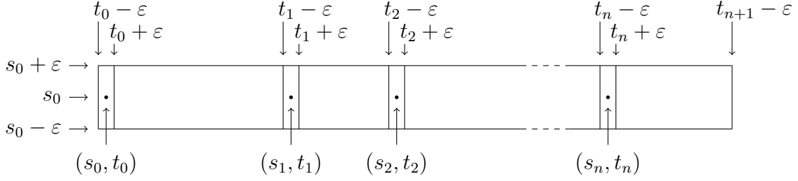
Figure 12: To compute \mathcal{W}_{s_0+\varepsilon}^{[t_0-\varepsilon, t_0-\varepsilon+l]}(\tilde{w}) - \mathcal{W}_{s_0-\varepsilon}^{[t_0-\varepsilon, t_0-\varepsilon+l]}(\tilde{w}) , we use winding numbers over the time intervals indicated in this Figure.
