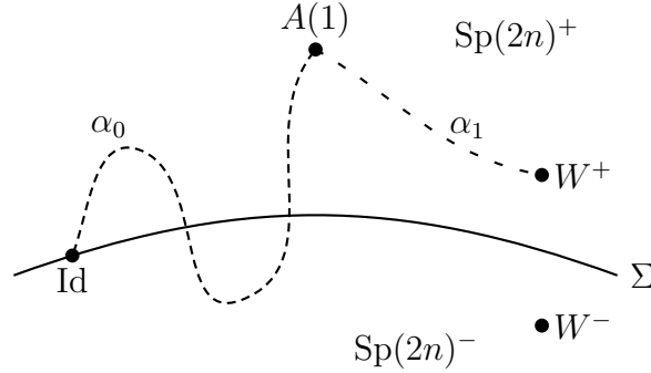
Figure 3: Path of symplectic matrices.
