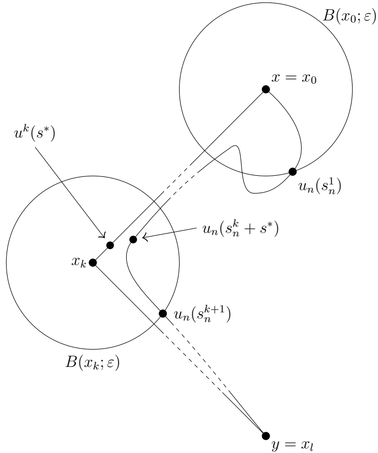
Figure 5: The illustration of how a sequence (u_n)_n of trajectories becomes a broken trajectory.
