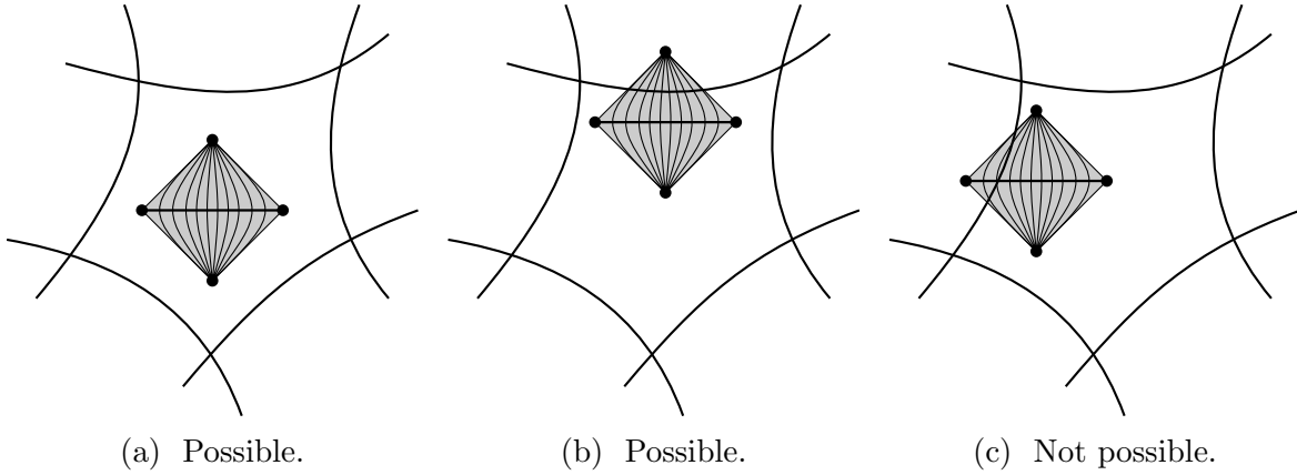
Figure 8: Proper braid class [X \text{ rel } Y] with more examples of spaces \mathcal{M}(U_-, U_+) .
